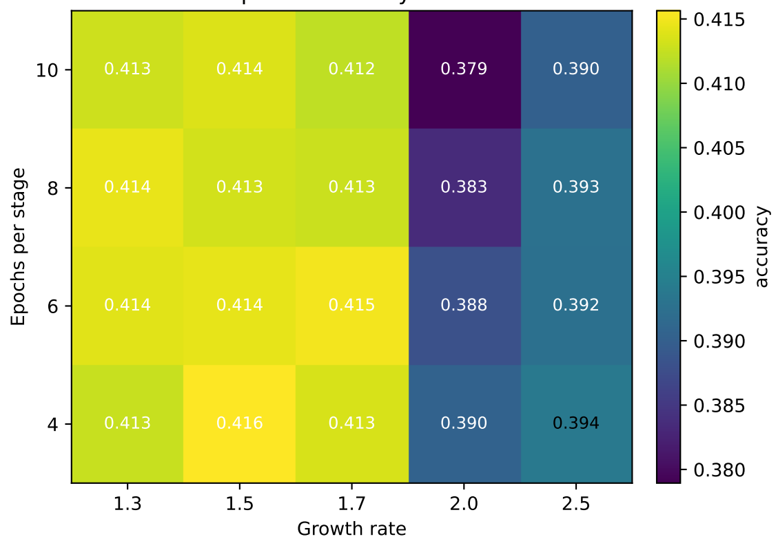
Linear probe accuracy — CIFAR10
