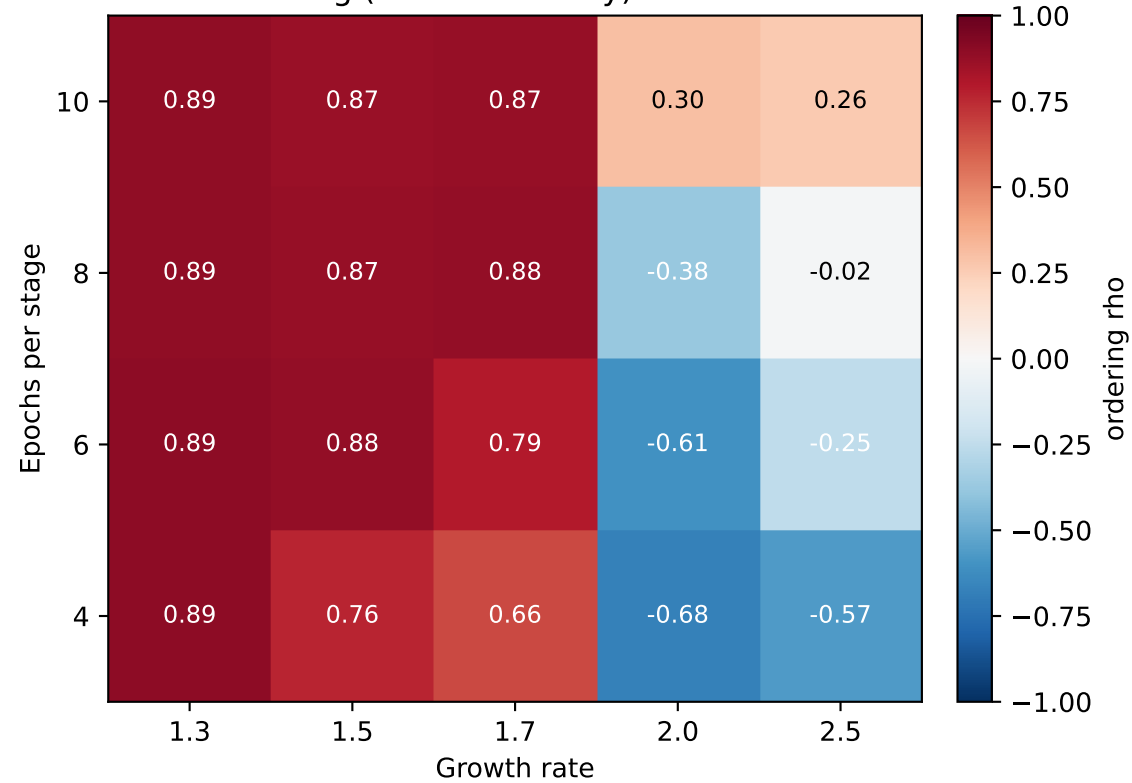
Ordering (variance-decay) — CIFAR10
