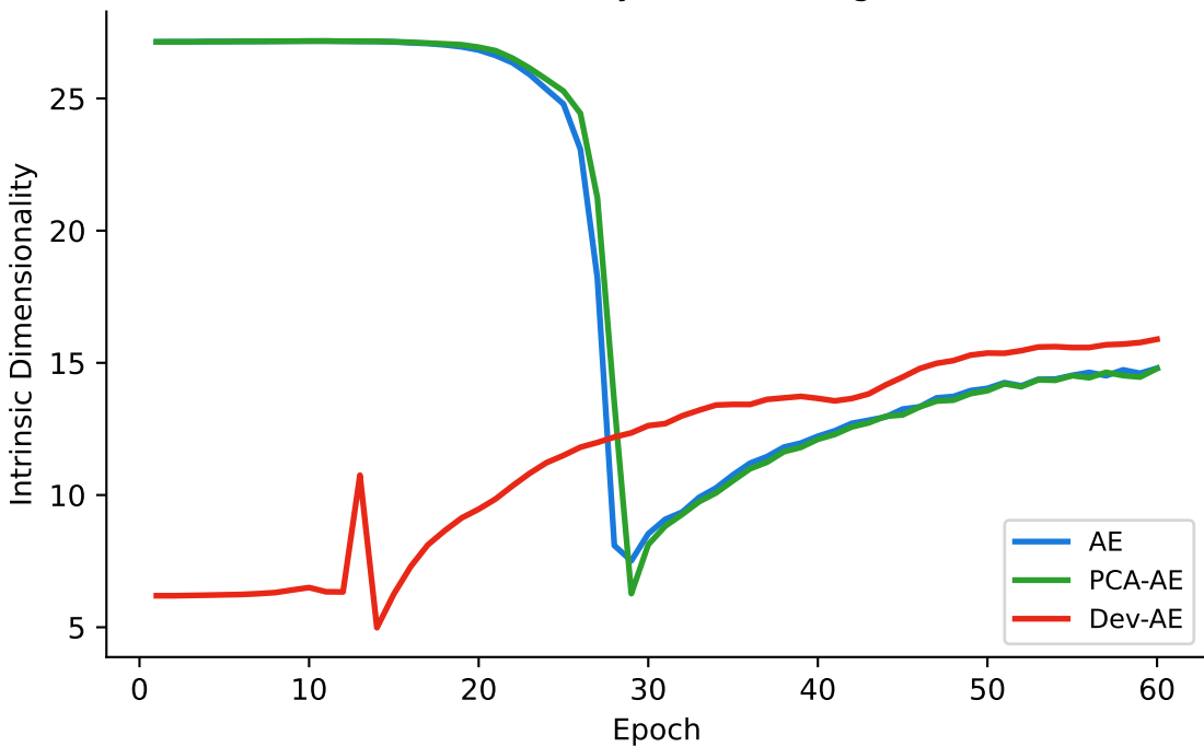
Latent dimensionality over training (CIFAR10)
