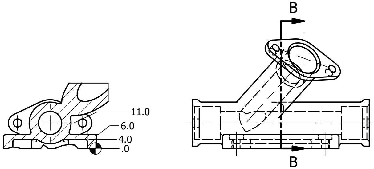
SECTION B-B SCALE 1 : 1
