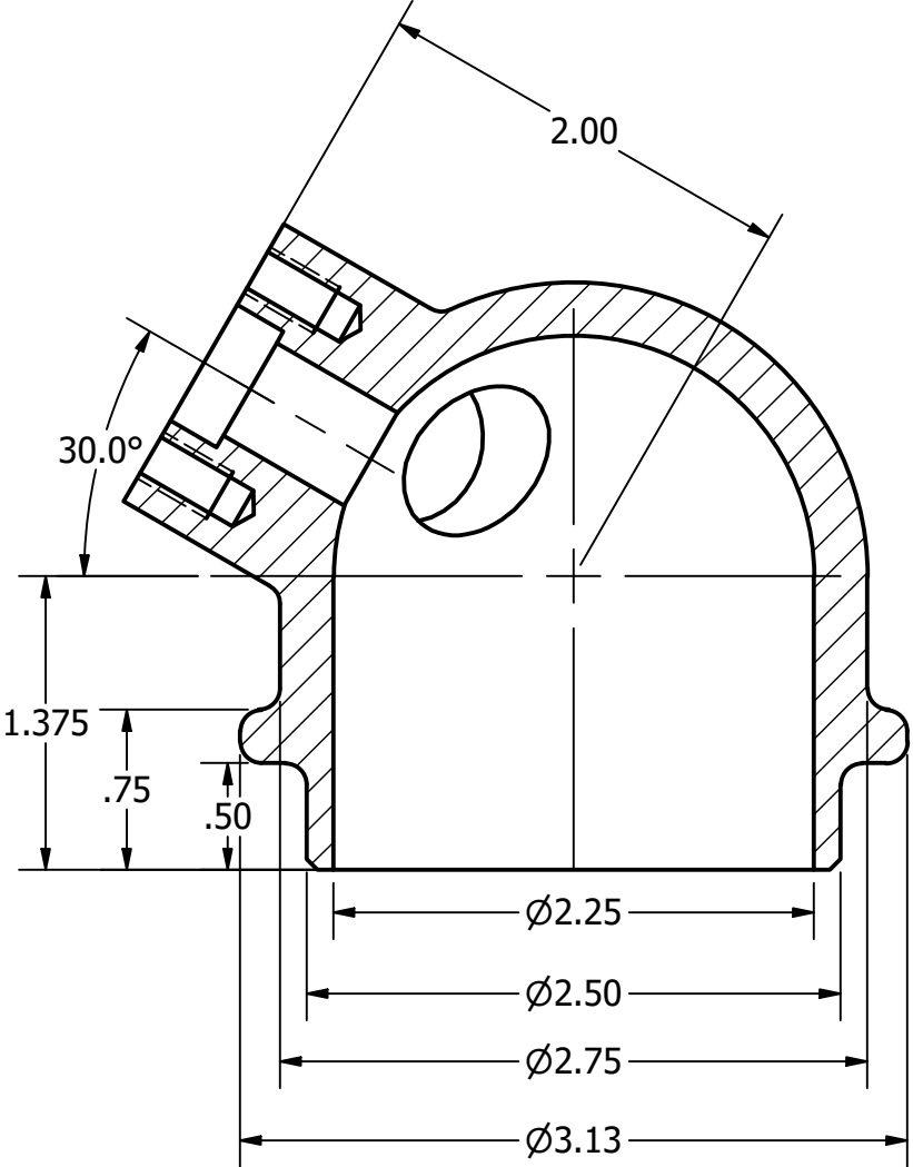
SECTION AA-AA SCALE 1 : 1
