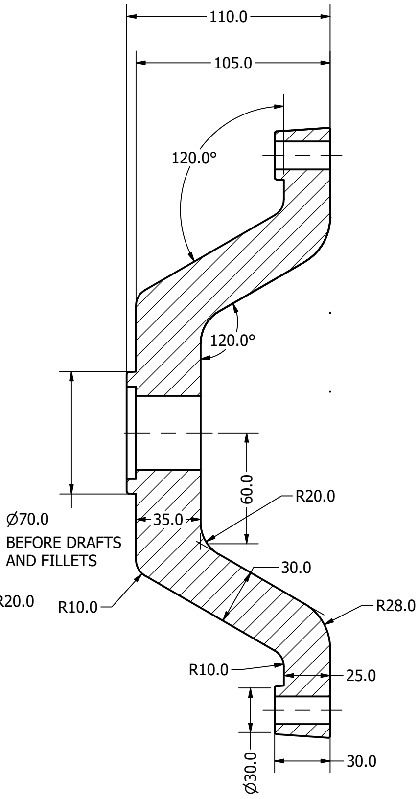
SECTION AU-AU SCALE 1 / 2
