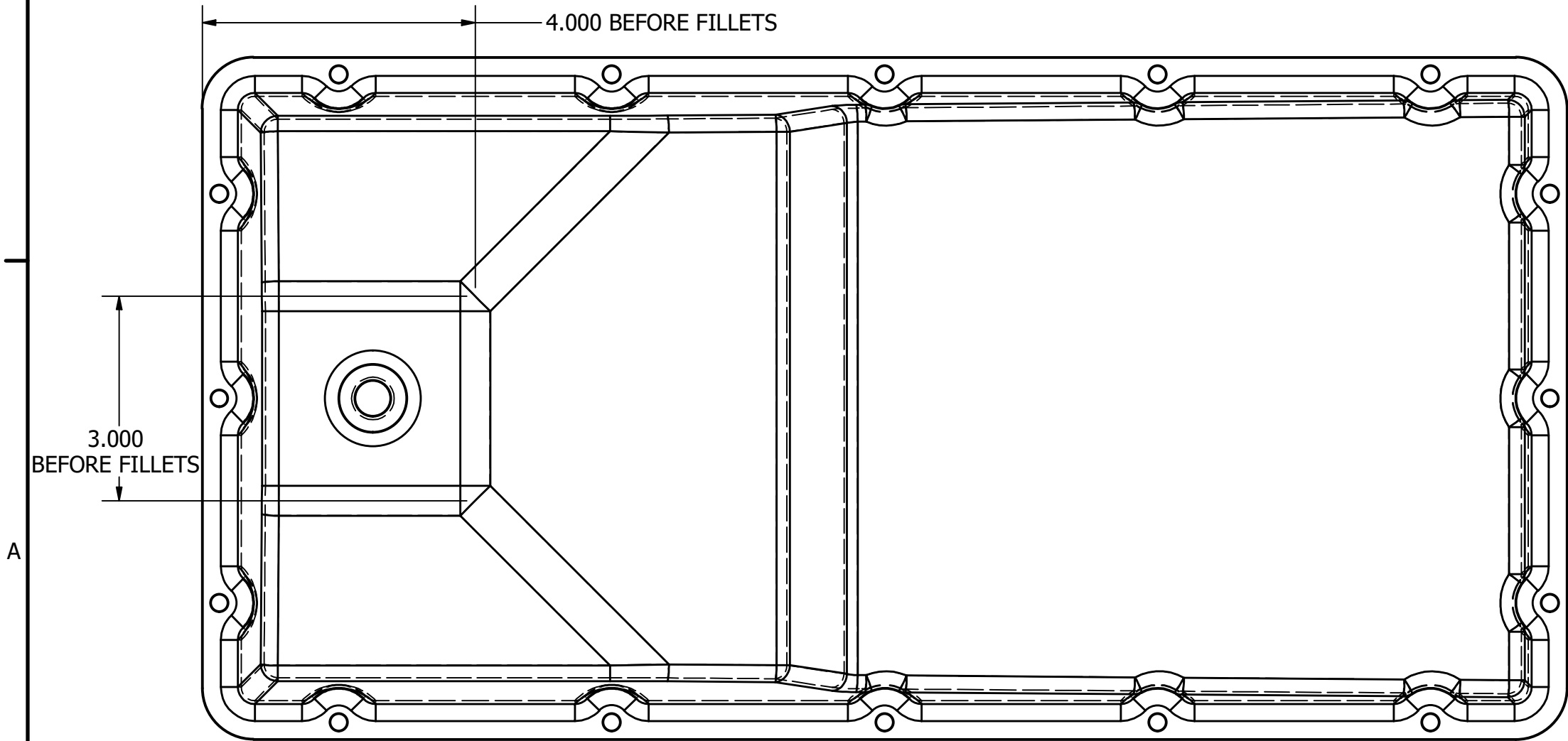
SECTION C-C SCALE 1/2
