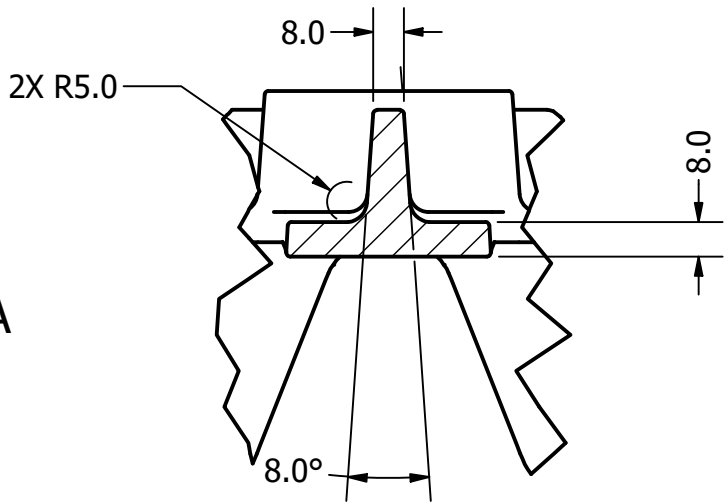
SECTION A-A SCALE 1 / 2
