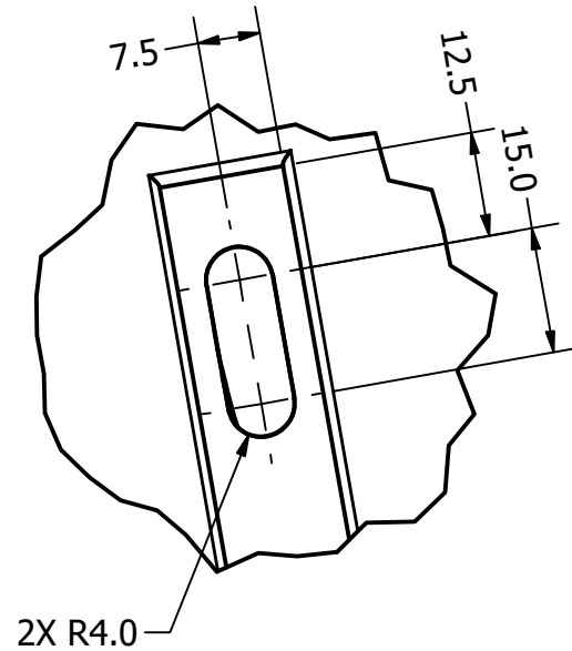
DETAIL F SCALE 1 : 1
