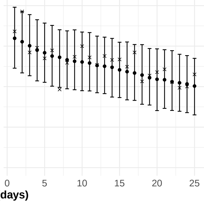
Neg. Bin. DLNM with temporal structures
