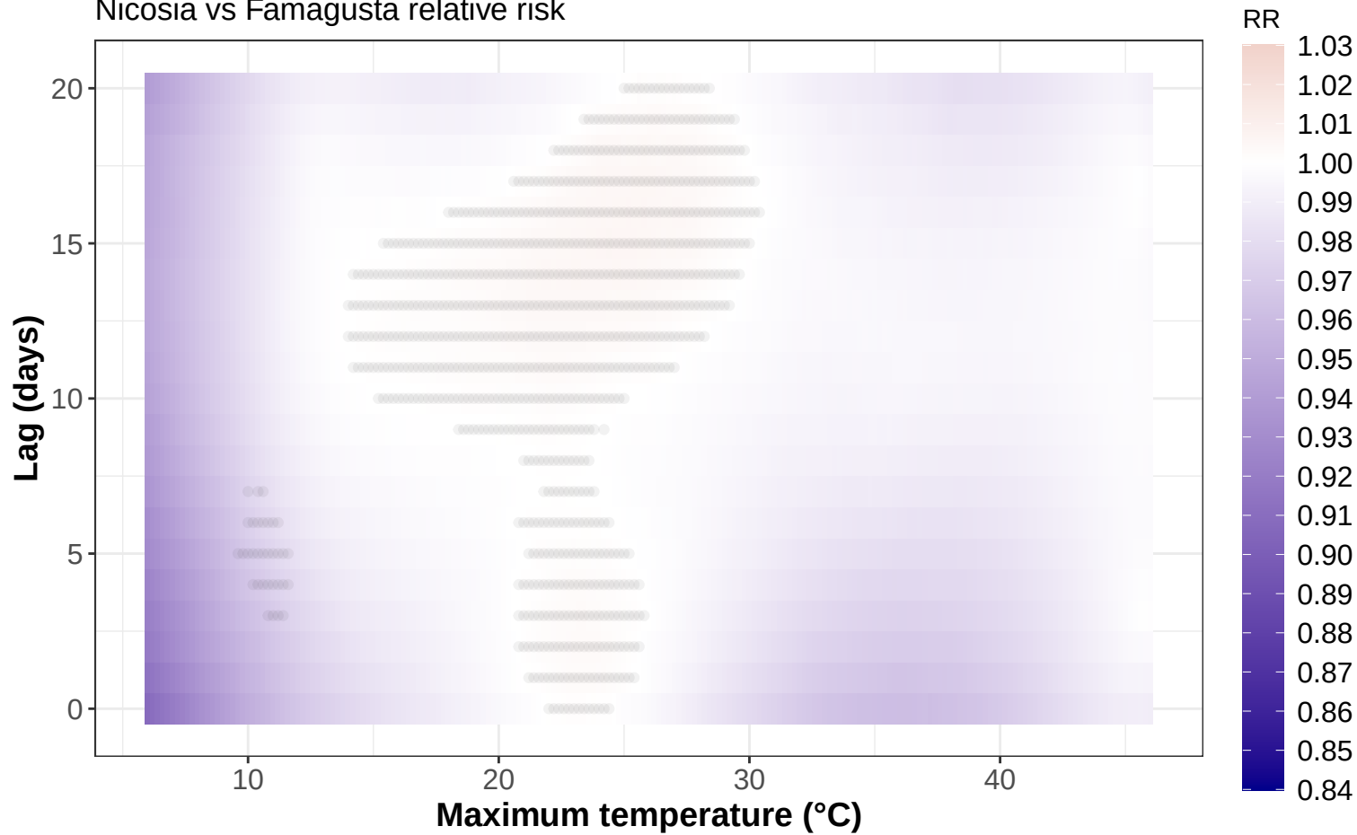
Nicosia vs Famagusta relative risk
