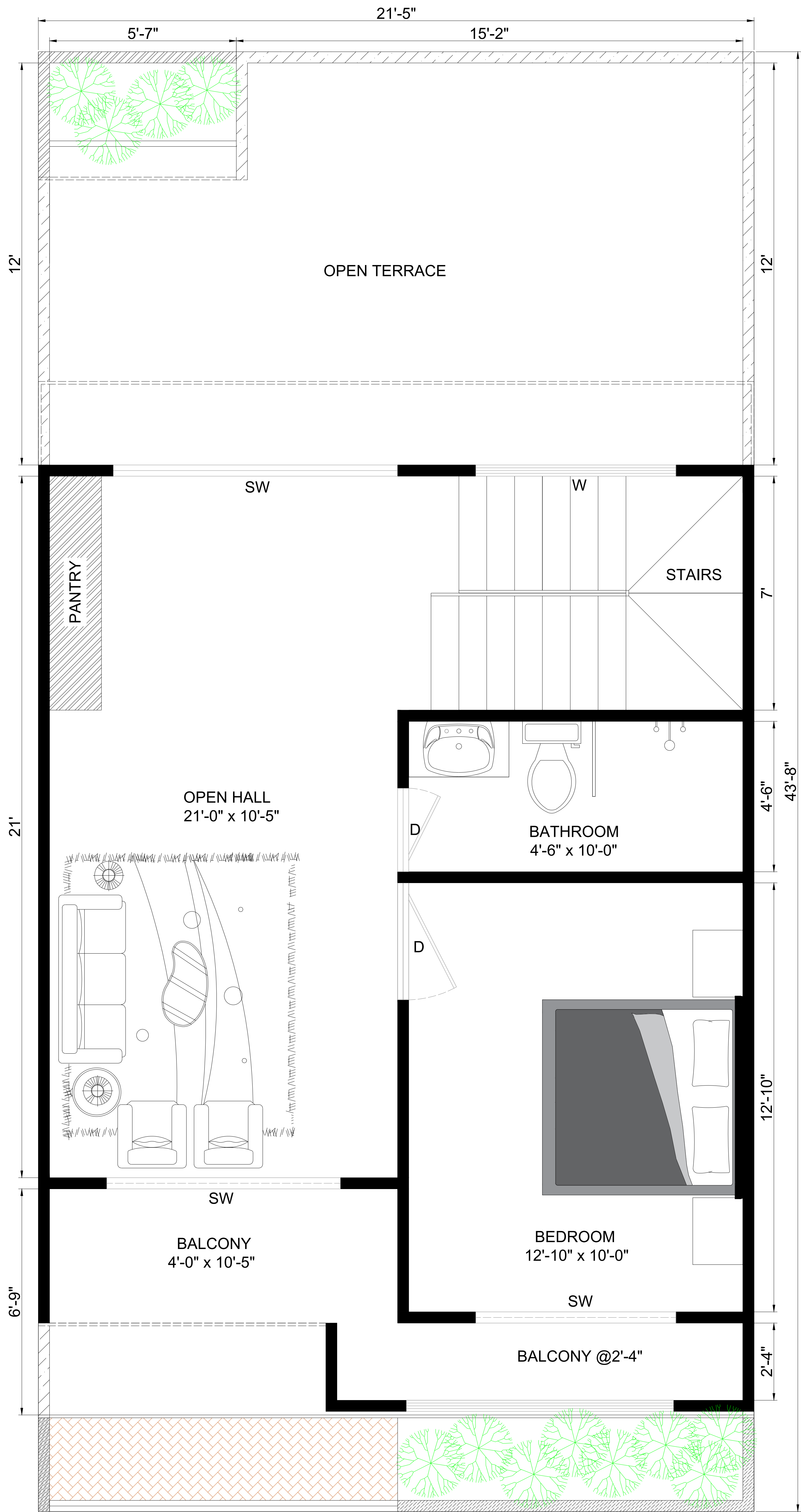
FIRST FLOOR 21'-5" X 43'-8"
