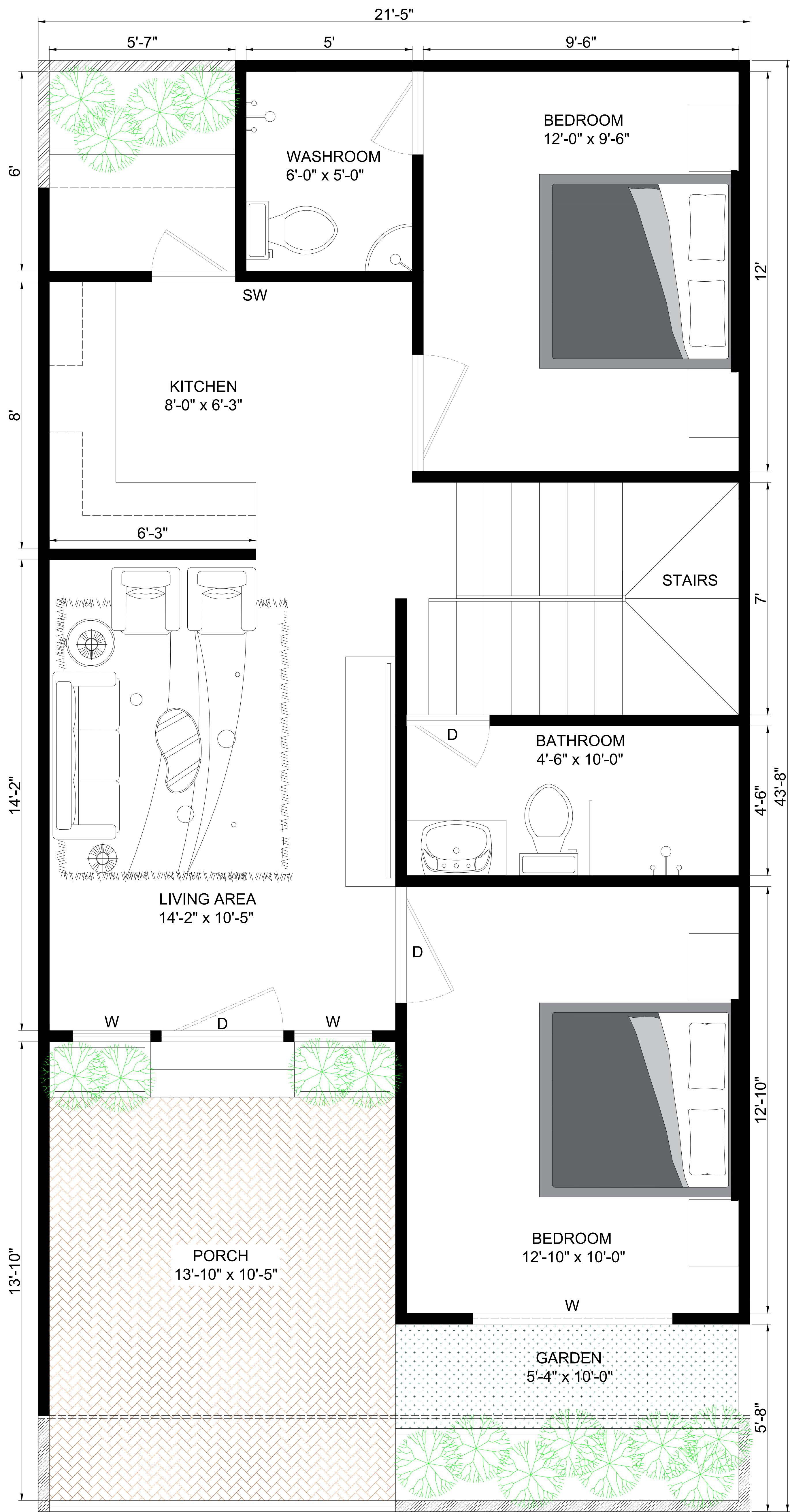
GROUND FLOOR 21'-5" X 43'-8"
