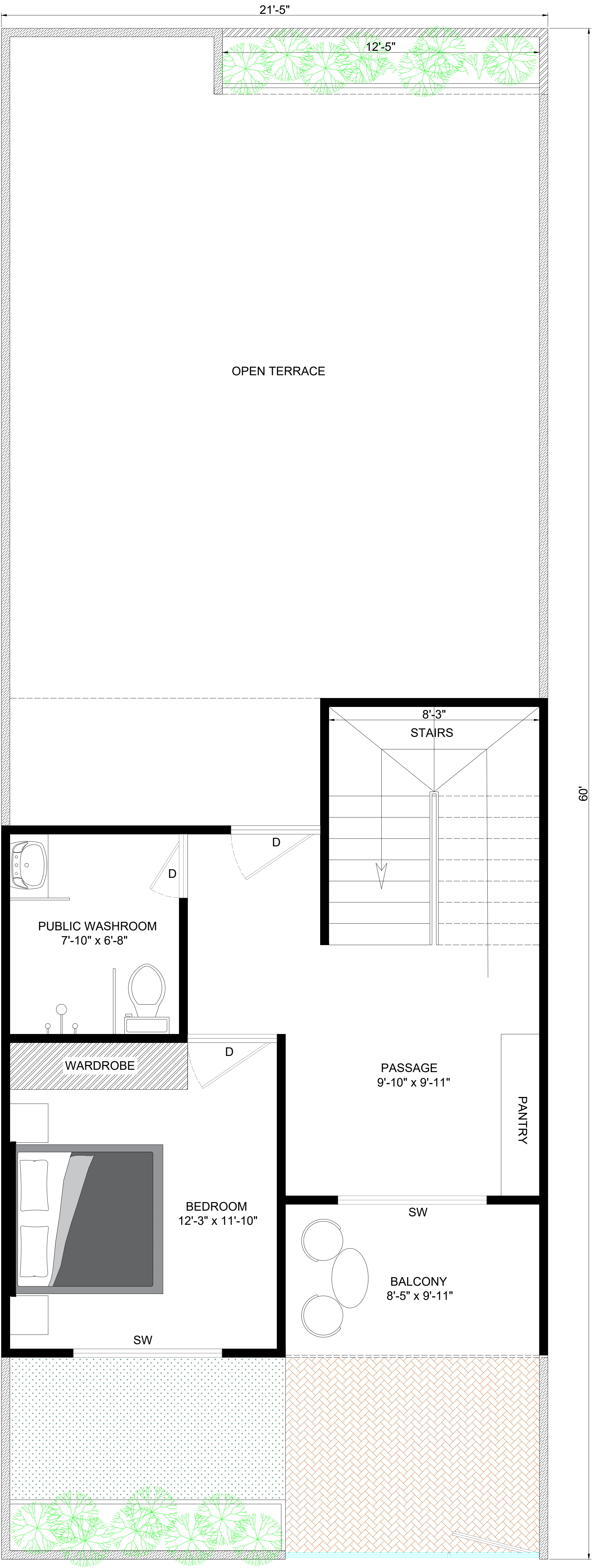
FIRST FLOOR 21'-5" X 60'-0"
