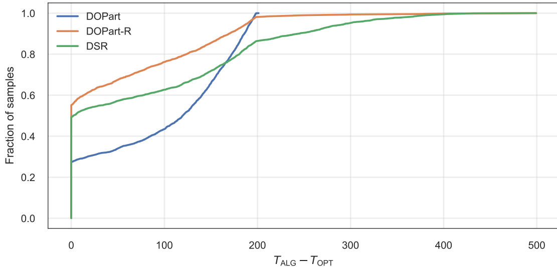
Regret CDF In The Volatile-Wireless Case
