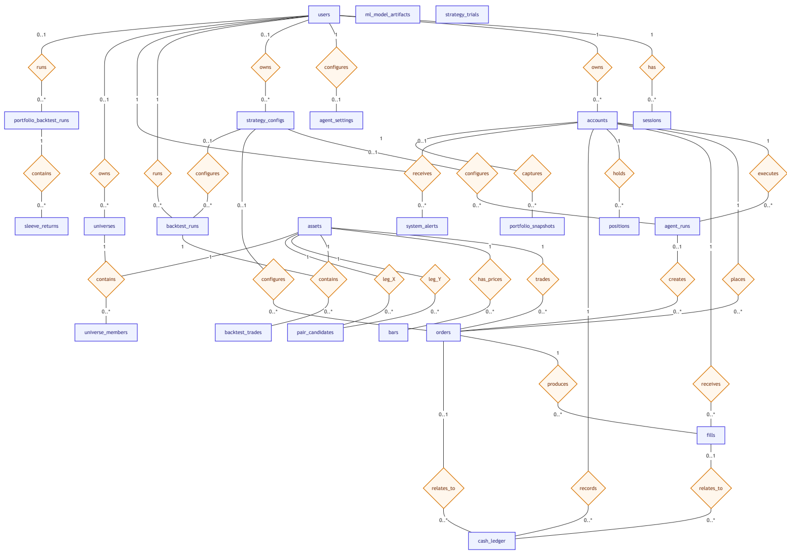
Entity-Relationship Diagram — Chen Notation
