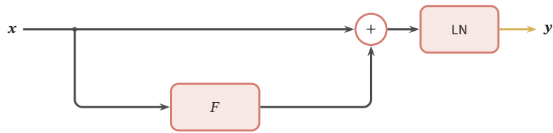
Post-LN
