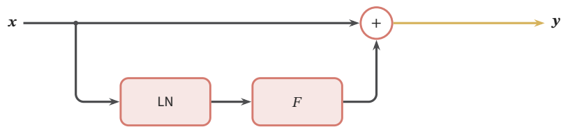
Pre-LN
