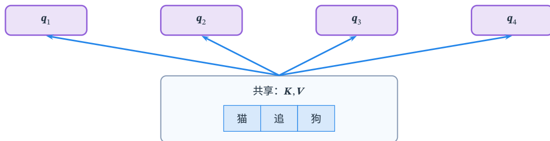
(c) MQA: 1 组键值
