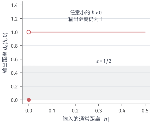
(b) \text{id}:(\mathbb{R}, d_u) \rightarrow (\mathbb{R}, d_d)
