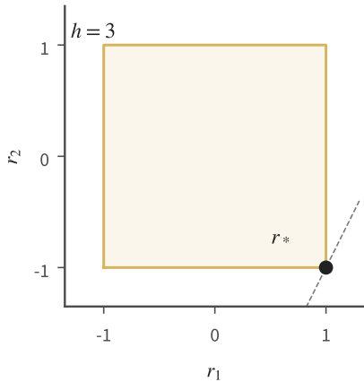
(c) \|r\|_\infty \leq 1
