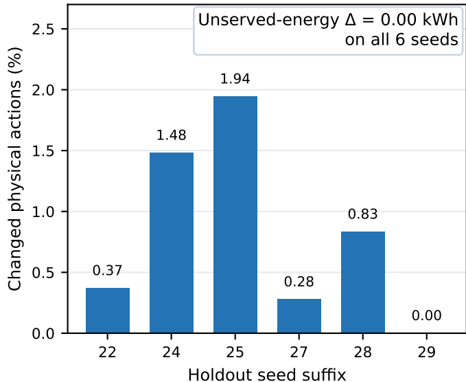
(b) Action change without shortage change
