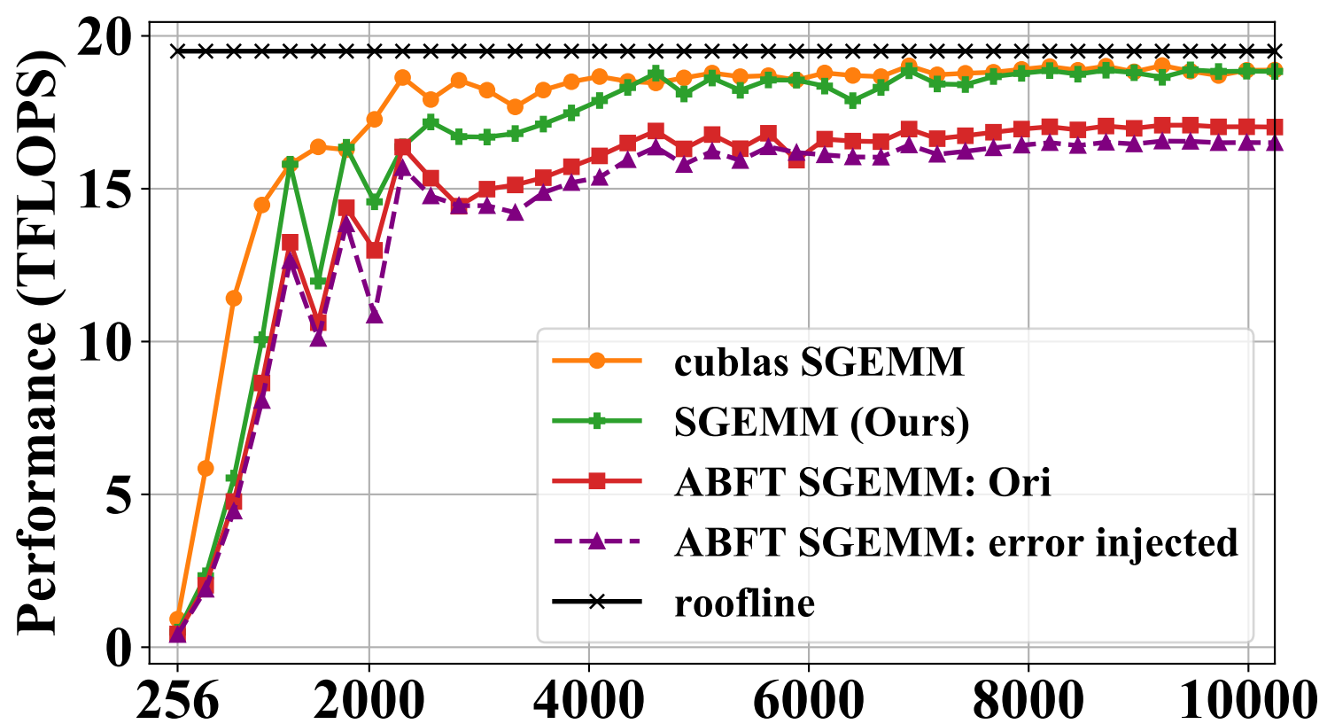
(a) Matrix Sizes M=N=K
