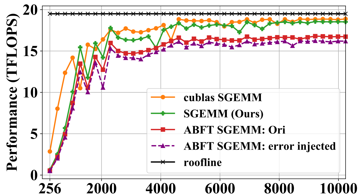
(b) Matrix Sizes M=K, K=1024
