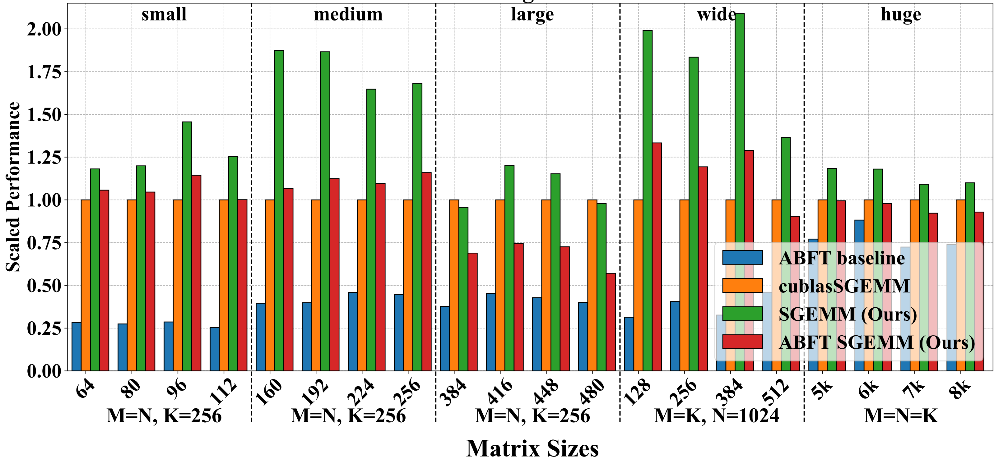
Performance of generated kernels
