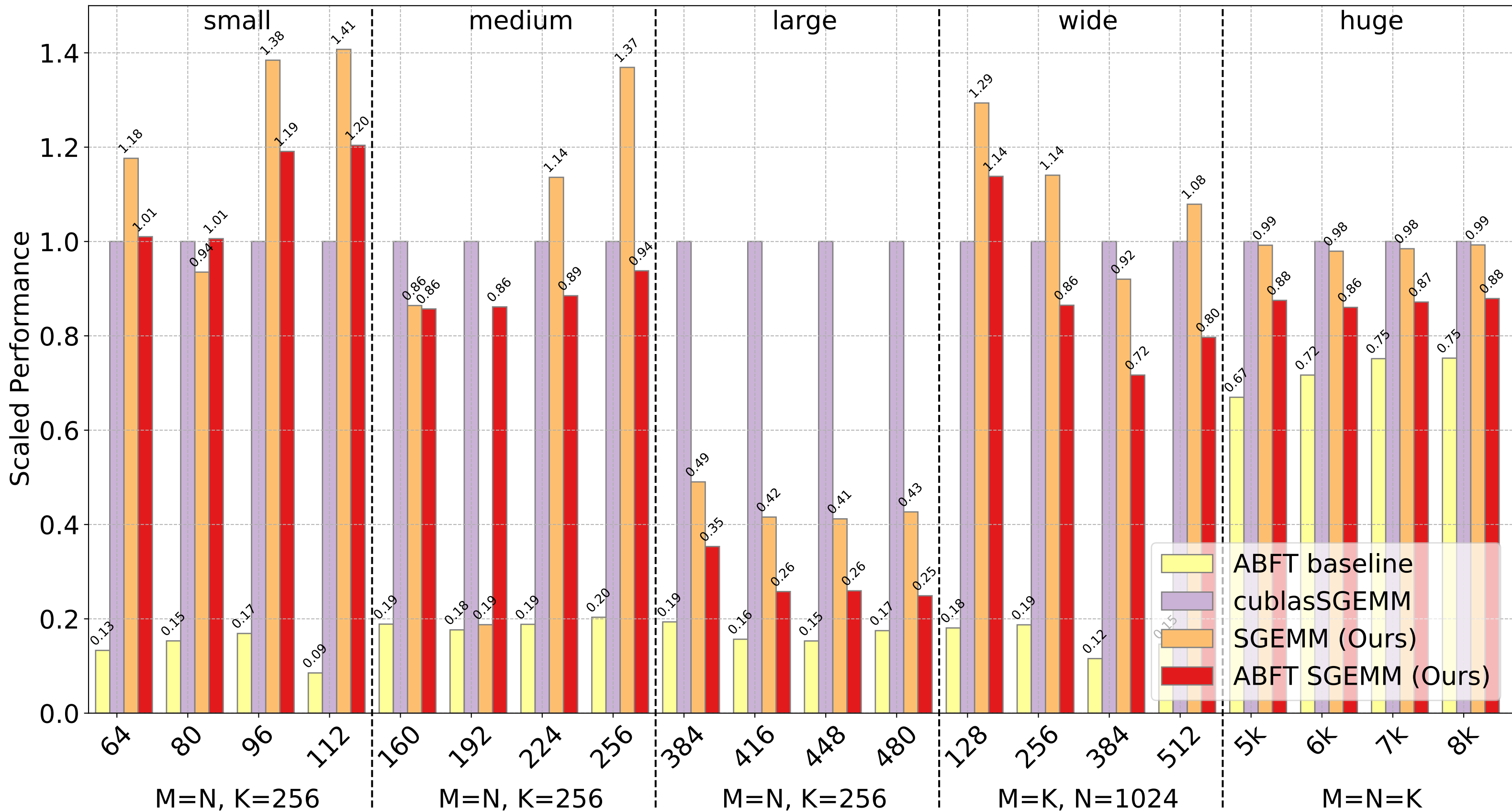
Performance of Generated Kernels on A100
