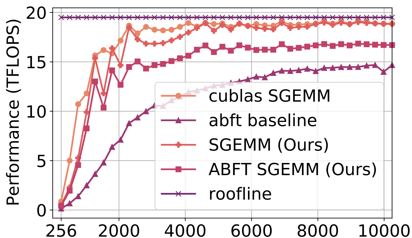
(a) Matrix Sizes M=N=K
