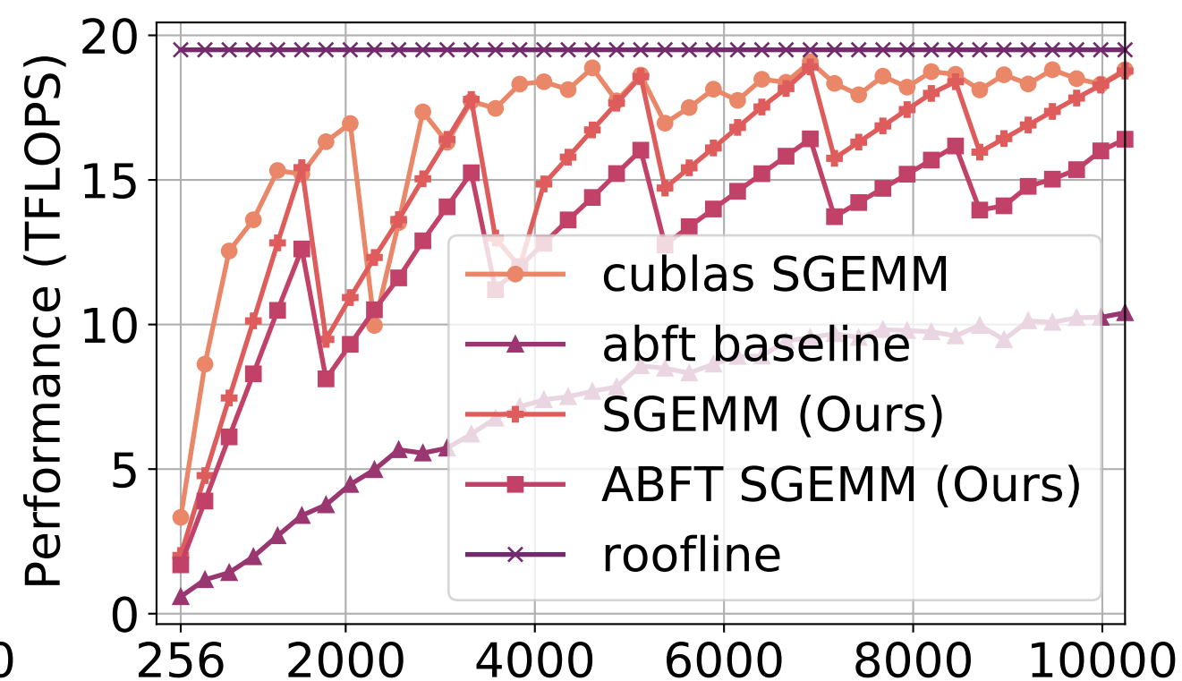
(b) Matrix Sizes M=K, N=1024
