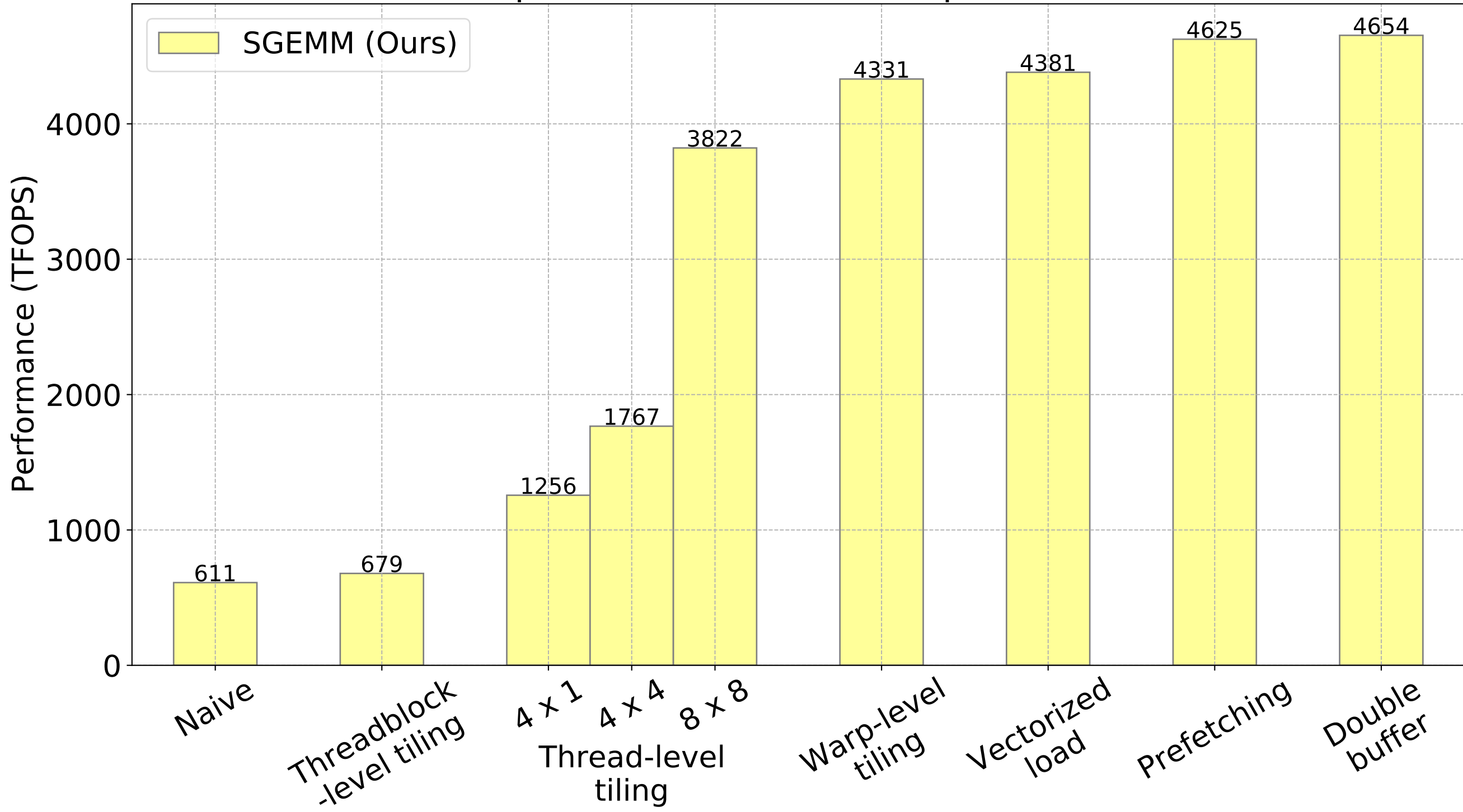
Step-wise SGEMM Kernel Optimization
