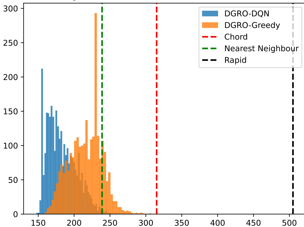
DGRO Training Performance: Diameter Distribution RL N=100 K=3
