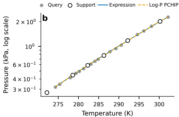
Vapor pressure: N-methylethylenediamine
