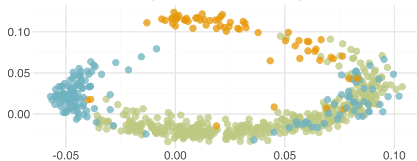
HyperGCN
