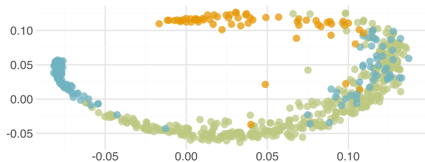
HGNN
