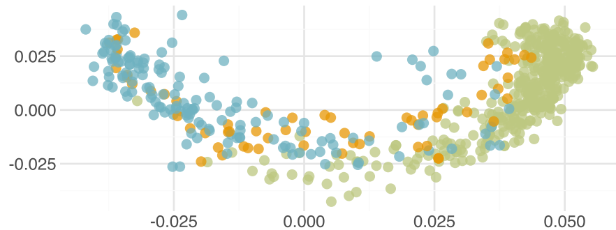
HGNN
