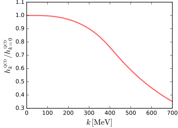
FIG. 6. Yukawa coupling, normalized to unity for k = 0 , as a function of the RG scale k , computed from the first-principles QCD within the fRG in the vacuum [10].
