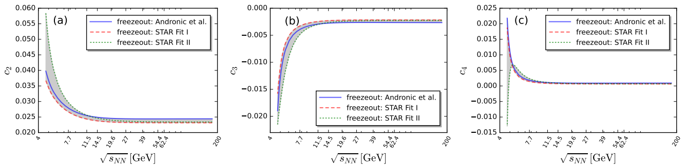
FIG. 5. Variance (panel a), skewness (panel b), and kurtosis (panel c) of temperature fluctuations, i.e., c_2 , c_3 and c_4 , as functions of the collision energy, calculated on the three representative freeze-out curves [22, 23, 66].
