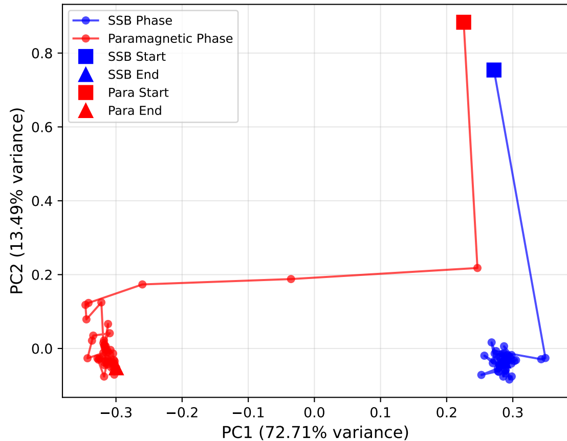
PCA of Average Latent Space
