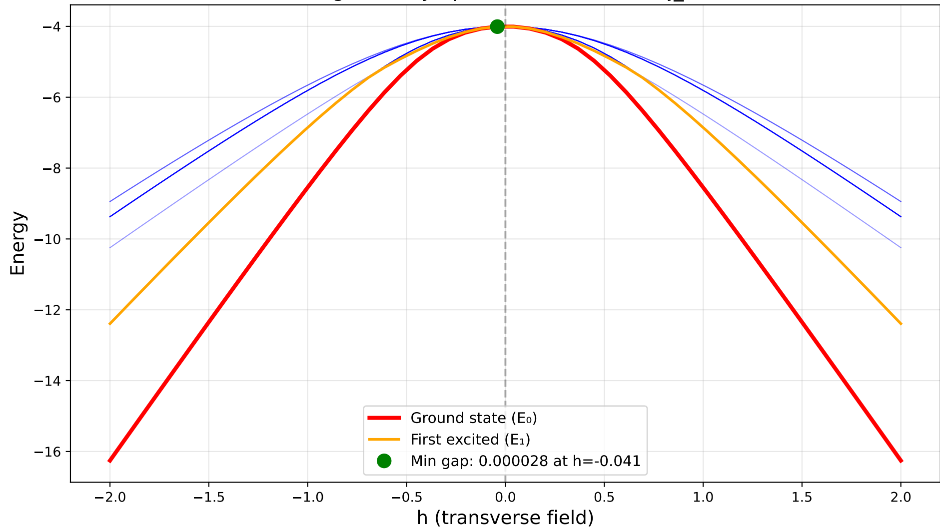
Z2 Gauge Theory Spectrum: 2x2 lattice, j_a=-1.0
