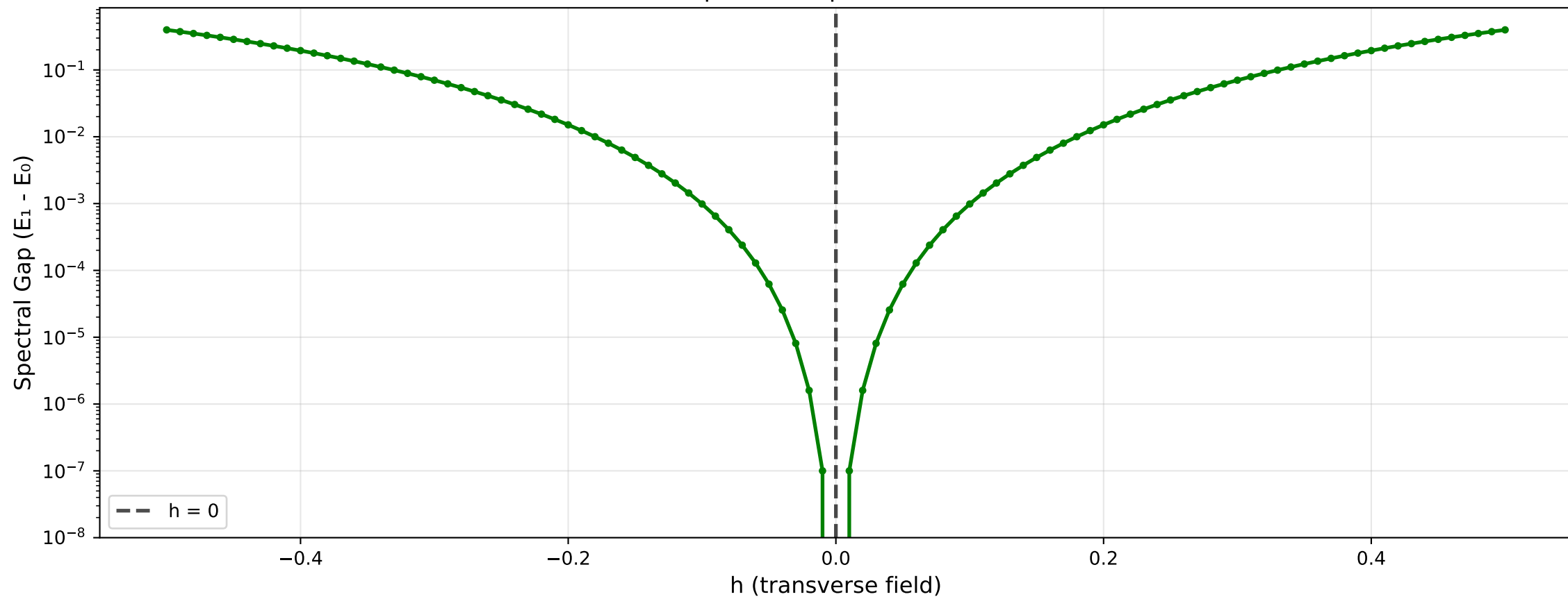
Spectral Gap Near h = 0
