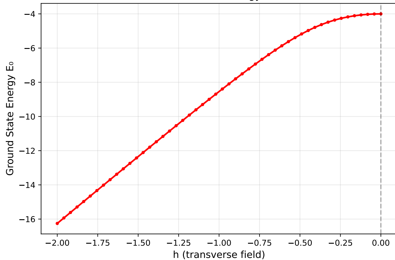
Ground State Energy vs h
