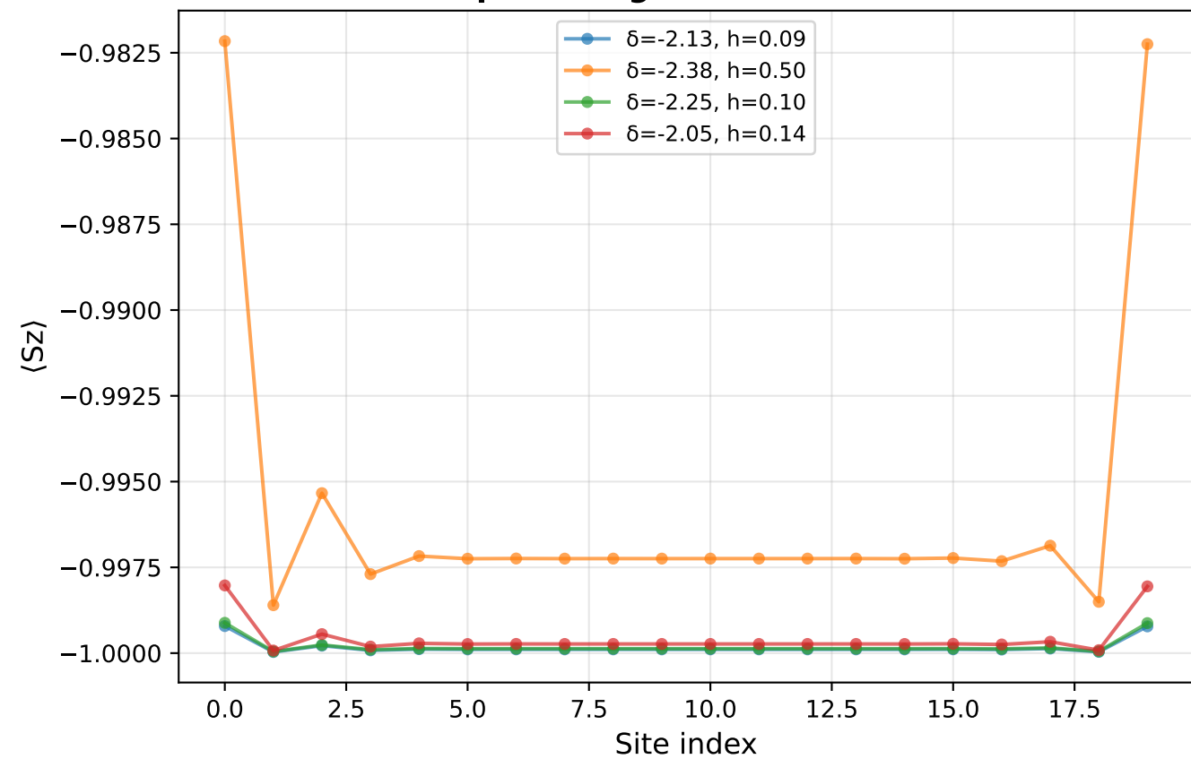
Sample Z-Magnetization Profiles
