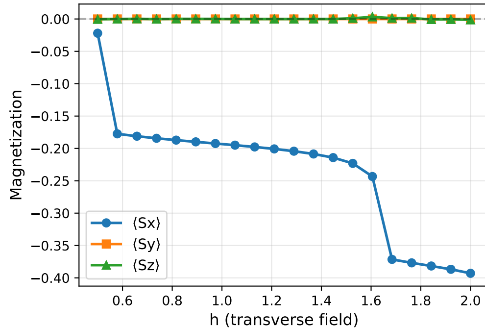
Magnetization vs h ( \Delta = 0.11 )
