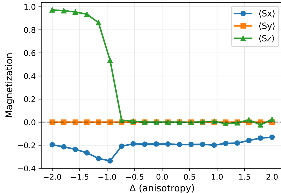
Magnetization vs \Delta ( h = 0.89 )
