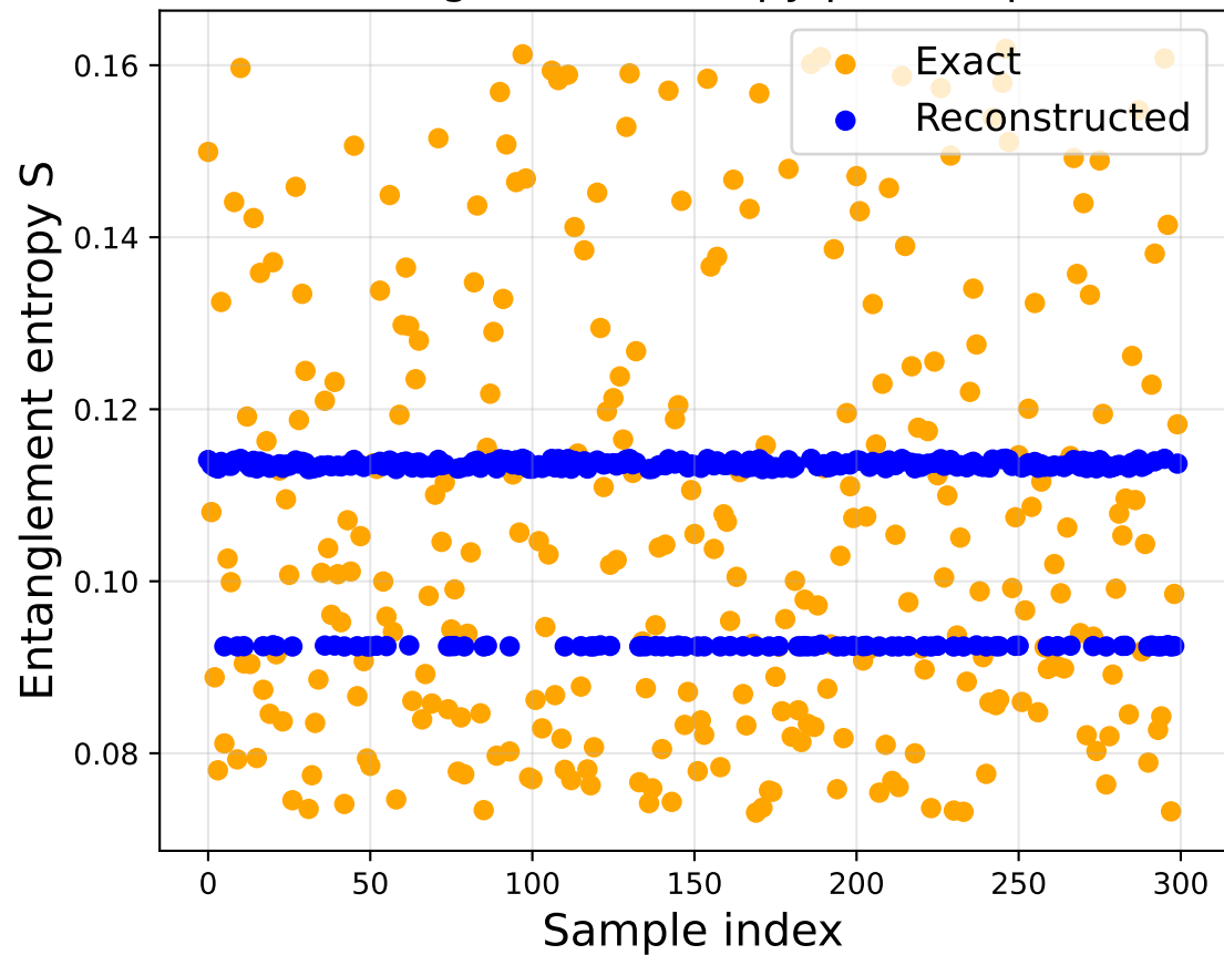
Entanglement entropy per sample
