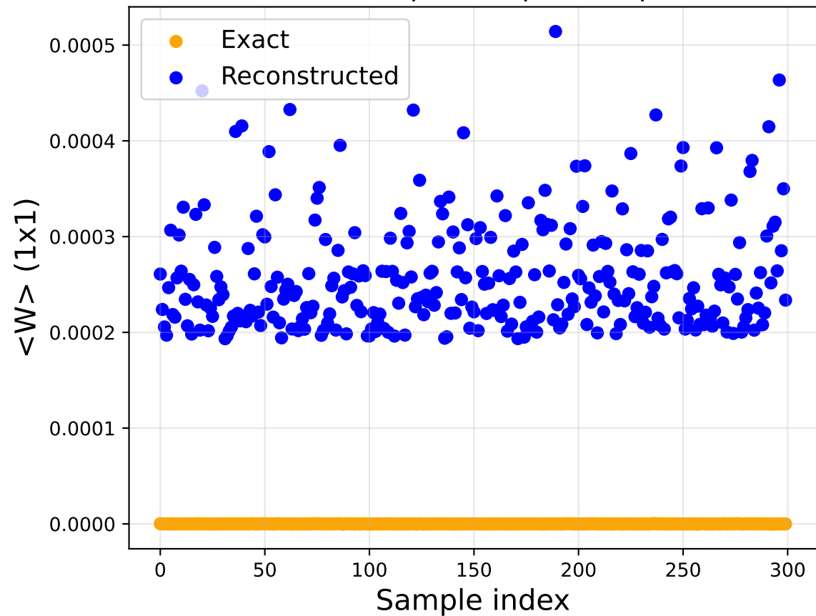
Wilson loop ( 1 \times 1 ) per sample
