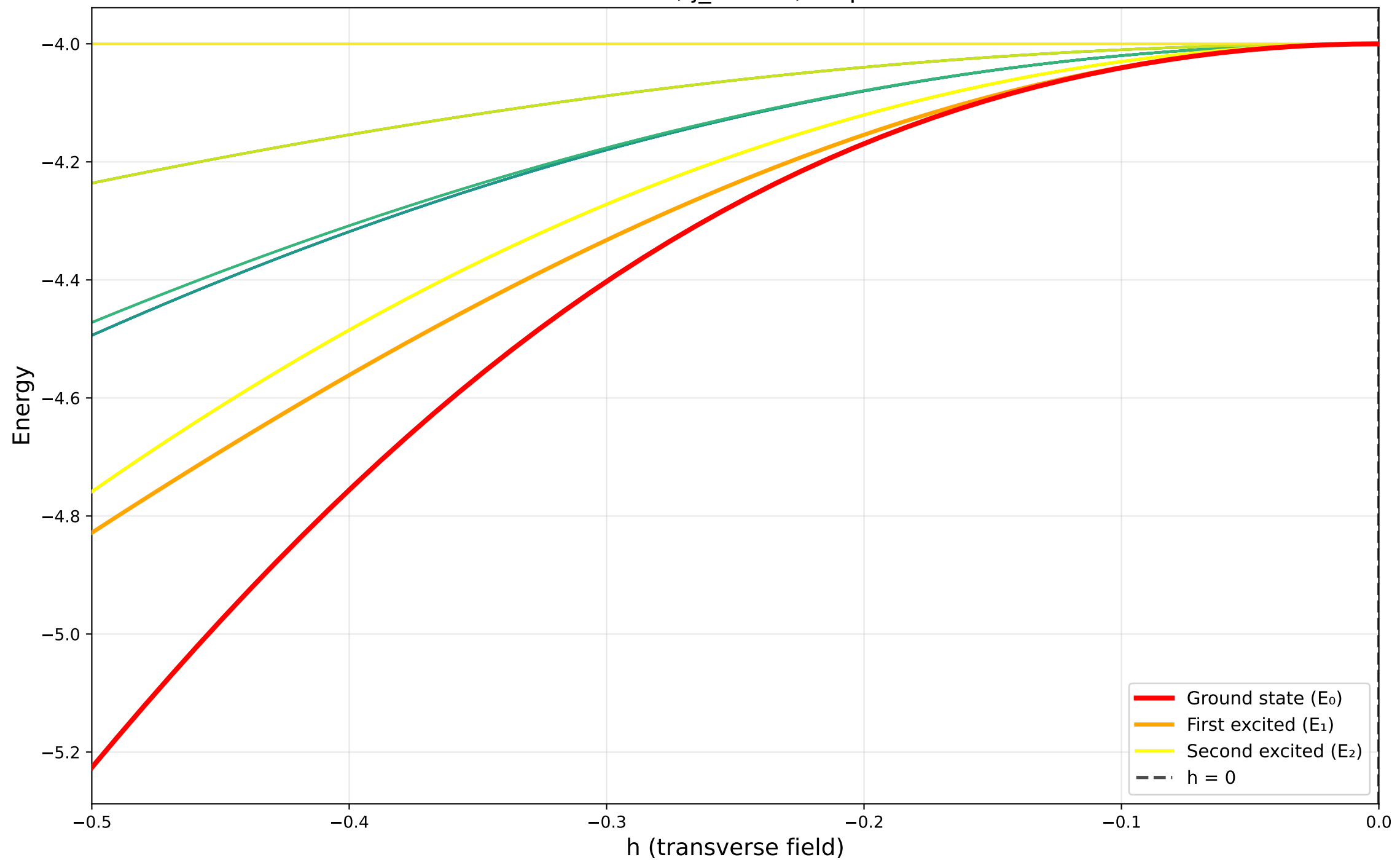
Lowest 32 Eigenvalues: h = -0.5 to 0 2x2 lattice, j_a = -1.0 , 50 points
