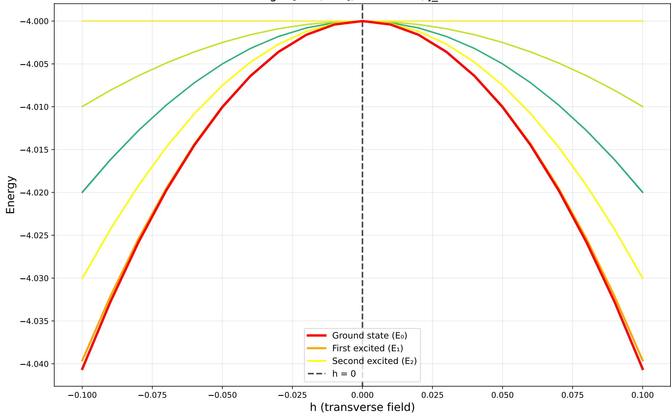
Lowest 32 Eigenvalues Near h = 0 (Zoomed) Range: [-0.1, 0.1] , 2 \times 2 lattice, j_a = -1.0
