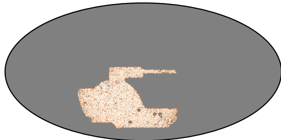
KS residual (unmasked)
