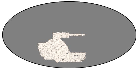
AKRA residual (unmasked)
