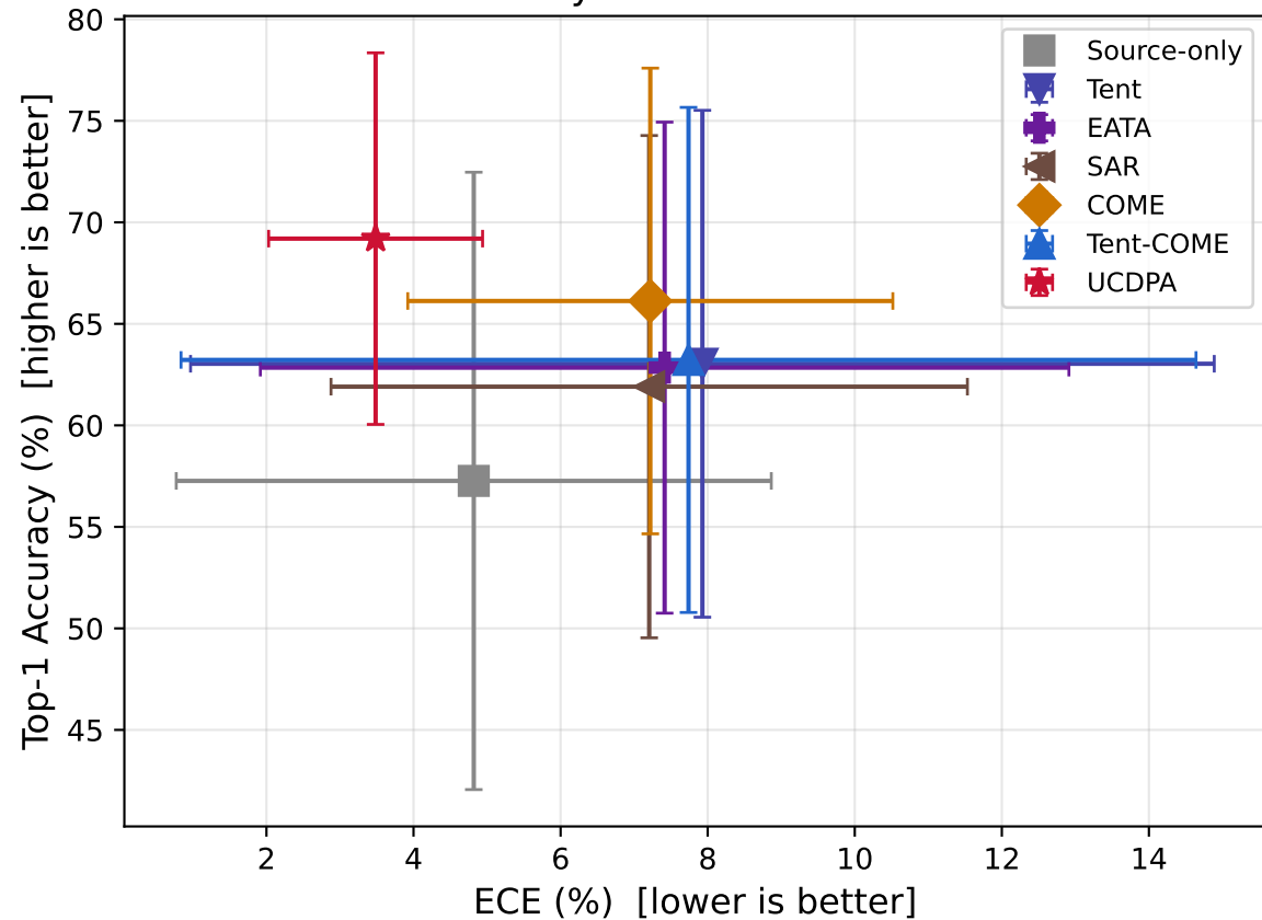
Accuracy vs Calibration Error
