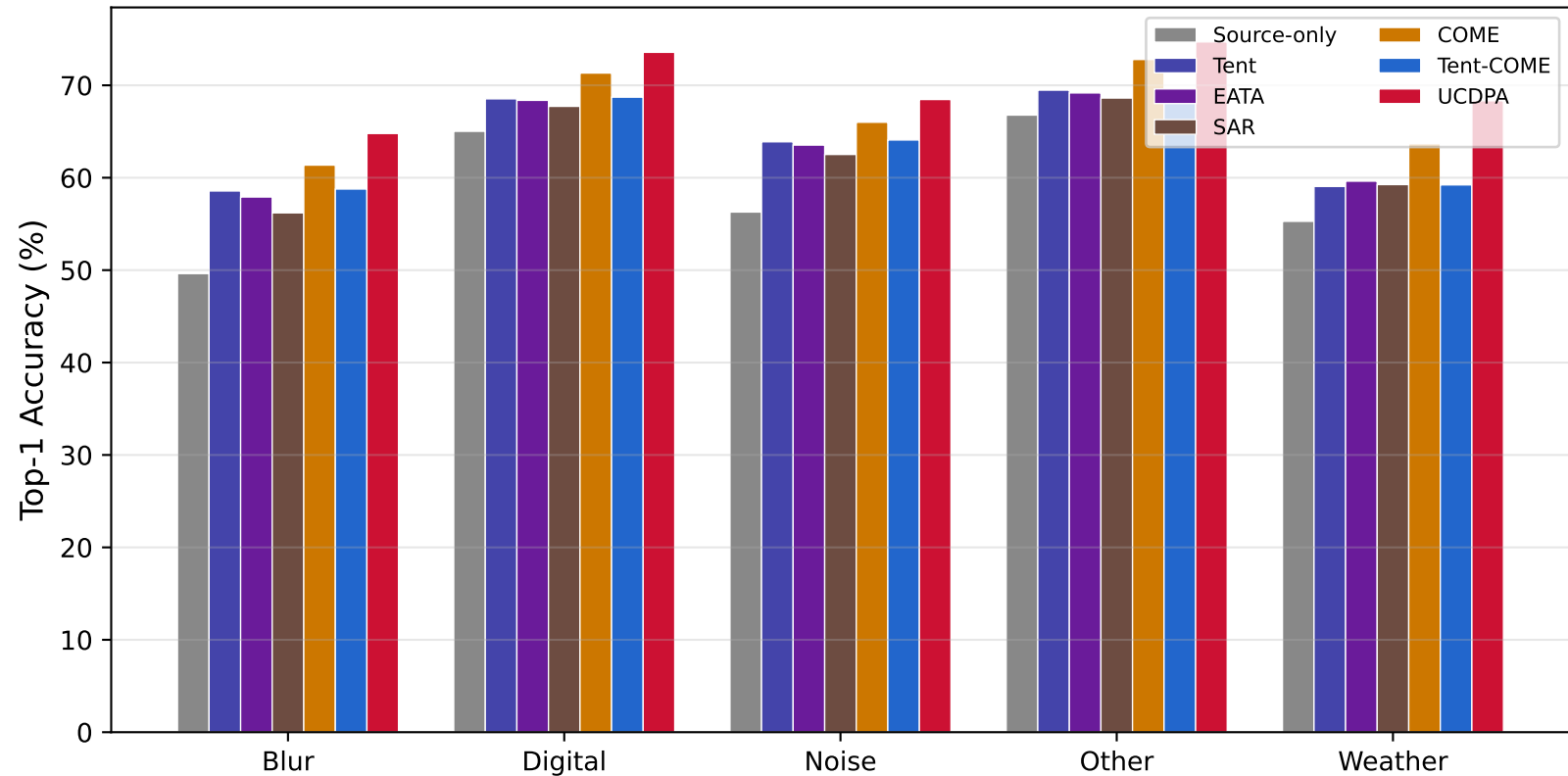
Accuracy by Corruption Family
