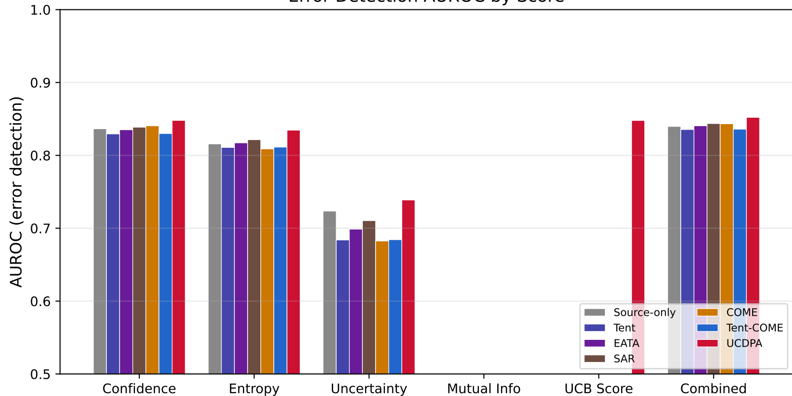
Error Detection AUROC by Score
