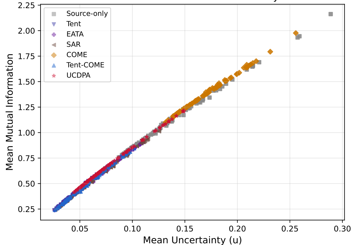
Mutual Information vs Uncertainty
