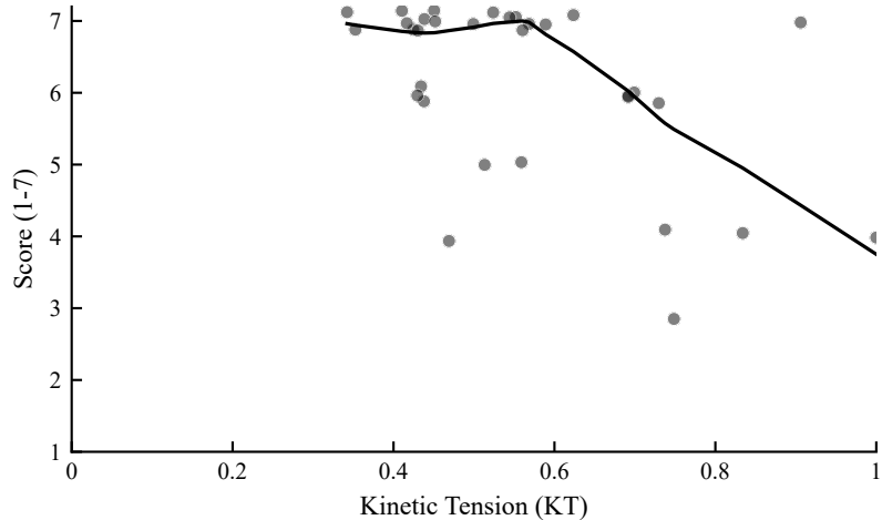
Temporal Mapping Perception ( \rho = -0.47 , p = 0.006 )
