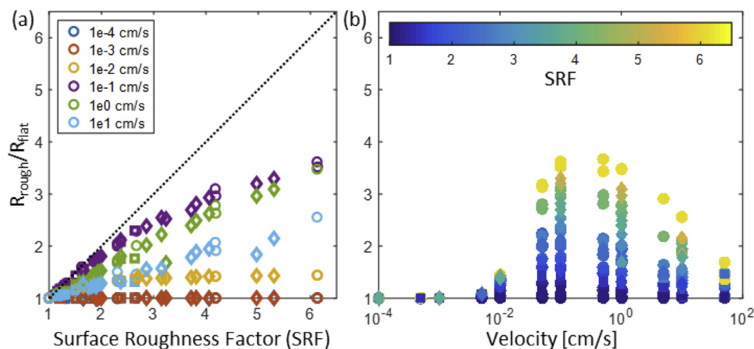
Fig. 4. The ratio between the reaction rate in a rough fracture and the reaction rate in a reference flat fracture in relation to (a) surface roughness factor and (b) flow velocities. The data points (○ – single sine wave profile, □ – self-similar profile, ◇ – self-affine profile) are results predicted by the roughness simulations. The hollow symbols in (a) are color-coded by velocity, and the filled symbols in (b) are color-coded by SRF.
