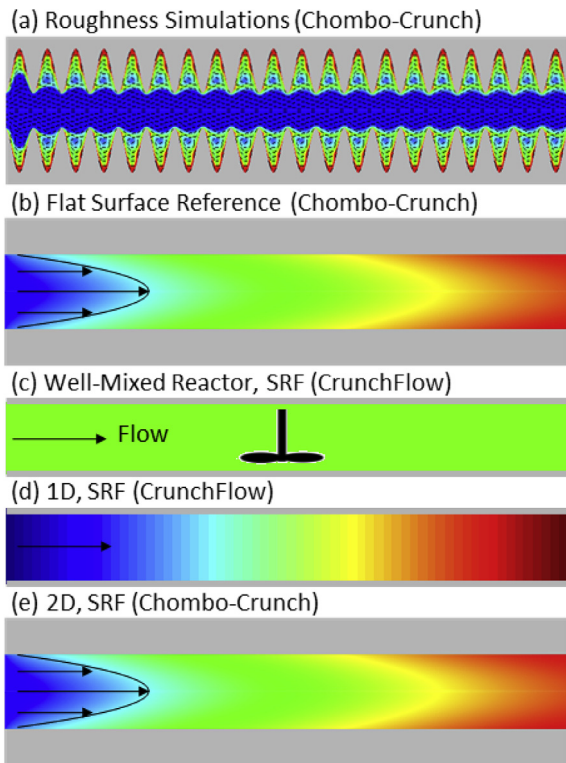
Fig. 2. Conceptual illustration of the different modeling approach and codes used in the simulations. (a) Roughness simulations using Chombo-Crunch, (b) a 2D flat-surface reference, (c) a well-mixed reactor, (d) a 1D model, and (e) a 2D model. Roughness in (a) and (b) is captured explicitly in the simulations, while SRF is used in (c)–(e). The color-map illustrates cation concentration with the warmer color corresponds to a higher concentration and the arrows indicate flow.
