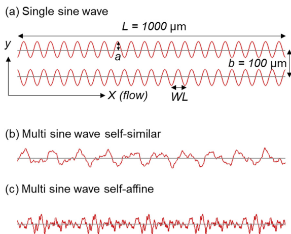
Fig. 1. (a) A rough fracture generated using a single sine wave with a wavelength of 50 \mu\text{m} and an amplitude of 30 \mu\text{m} . (b) A self-similar rough profile (lower half of the fracture) generated by overlaying 20 sine waves with wavelengths ranging from 0.0005 to 100 \mu\text{m} , and an amplitude-to-wavelength ratio of 0.2 . (c) A self-affine rough profile (lower half of the fracture) generated by overlaying 43 sine waves with wavelengths ranging from 4.35 to 50 \mu\text{m} , and an amplitude-to-wavelength ratio of 0.2 .
