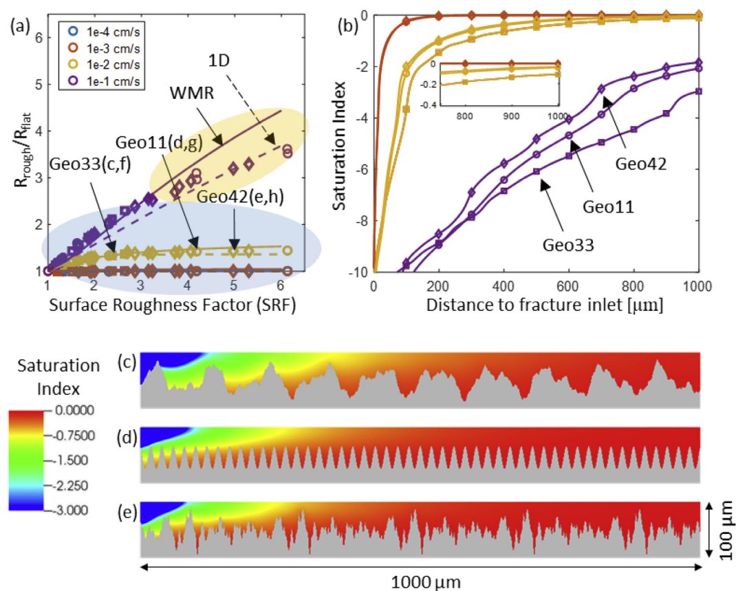
Fig. 5. (a) The ratio between the reaction rate over a rough profile and the rate over a flat profile plotted against surface roughness factor at velocities ranging from 0.0001 to 0.1 cm/s. The data points (○ – single sine wave profile, □ – self-similar profile, ◇ – self-affine profile) are results predicted by the roughness simulations. The solid lines plot the results from the well-mixed reactor, and the dashed line is the 1D results. The blue oval and yellow oval highlight the data points of roughness simulations that agree well with the well-mixed reactor simulations and the 1D simulations, respectively. (b) Saturation index at the center of the fracture for geometric profile 33 (□), 11 (○), and 42 (◇) at velocities of 0.001, 0.01, 0.1 cm/s (using the same color-code as (a)). (c–e) Color maps of the saturation index with respect to calcite at 0.01 cm/s in geometric profile 33, 11, and 42, respectively.
