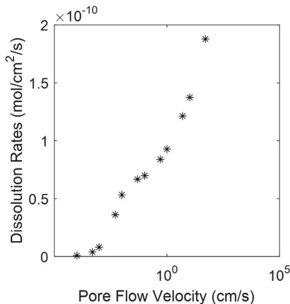
Fig. 3. Calcite dissolution rate of the reference flat fracture. The reaction rate is normalized against the geometric surface area.
