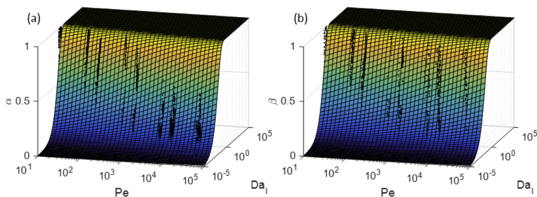
Fig. 9. (a) The multiplying factor ( \alpha ), and (b) the exponent ( \beta ) in relation to Pe and Da_I . The black dots are data points from the pore-scale reactive transport simulations.
