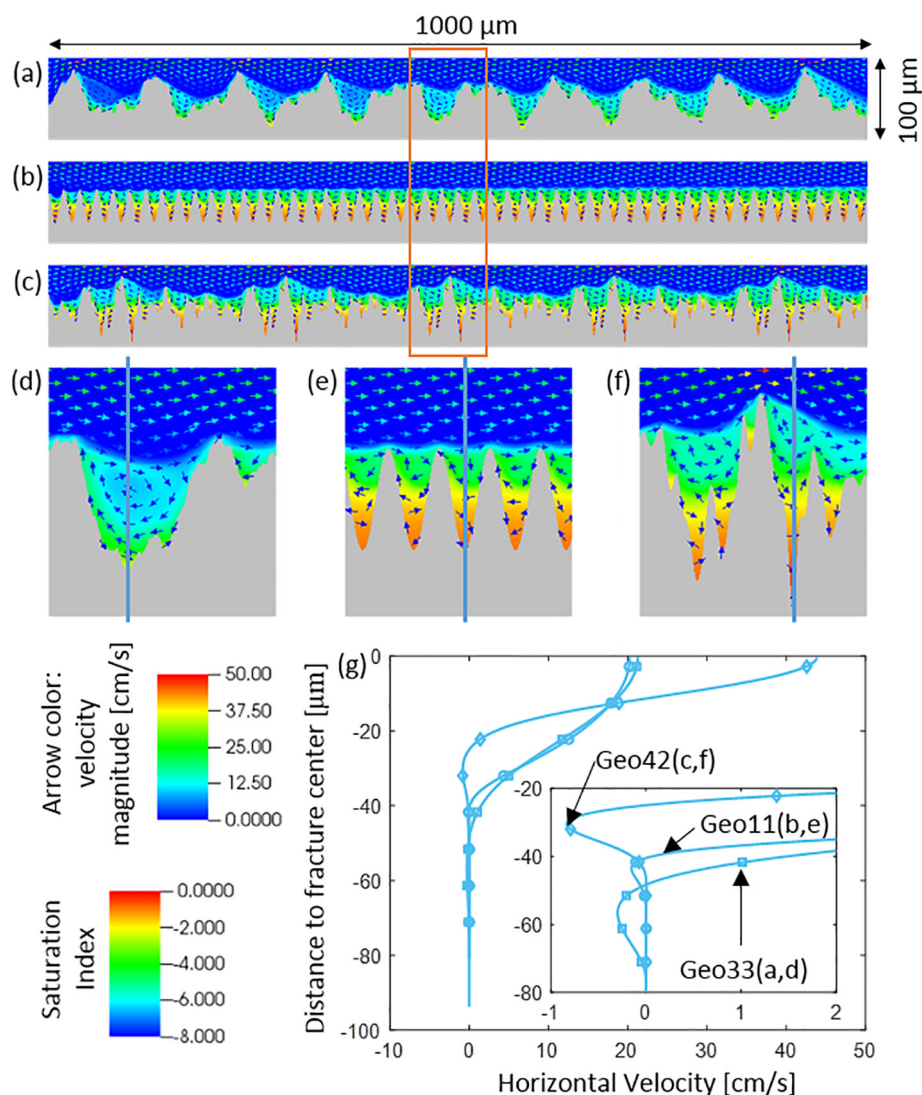
Fig. 7. (a–c) Saturation index and velocity vector at 10 cm/s for geometric profile 33, 11, and 42, respectively. (d–f) Blow-ups of the regions highlighted in orange in (a–c). (g) Horizontal velocity of the cross sections highlighted in (d–f) for geometric profile 33 ( \square ), 11 ( \circ ), and 42 ( \diamond ). Negative velocity indicates the change of flow direction.
