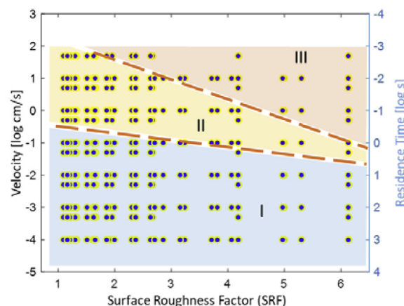
Fig. 8. Data points of the full length fracture simulations (black dots with yellow edge) plotted against surface roughness factor and average velocity [cm/s] and residence time [s]. The shaded areas illustrate the three regimes regarding the impacts of surface roughness on reaction rates with the same color code as Figs. 5 and 6.
