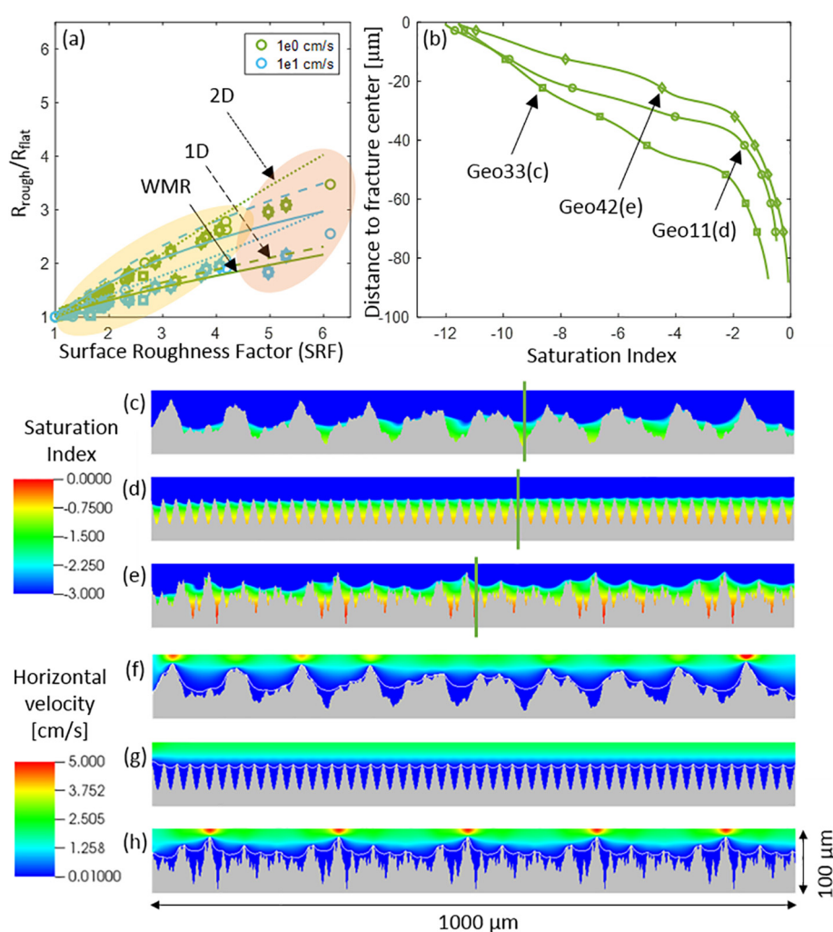
Fig. 6. (a) The ratio between the reaction rate over a rough profile and the rate over a flat profile plotted against surface roughness factor at velocities 1 and 10 cm/s. The data points ( \circ – single sine wave profile, \square – self-similar profile, \diamond – self-affine profile) are results predicted by the roughness simulations. The solid lines, dashed lines and dotted lines are results from the well-mixed reactor, 1D and 2D simulations, respectively. The yellow oval and orange oval highlight the data points of roughness simulations that agree well with the 1D and 2D simulations, respectively. (b) Saturation index from the center of the fracture to the fracture surface at 1 cm/s for geometric profile 33 ( \square ), 11 ( \circ ), and 42 ( \diamond ) at the location highlighted in (c–e). (c–e) Color maps of saturation index with respect to calcite at 1 cm/s in geometric profile 33, 11, and 42, respectively. (f–h) Color maps of horizontal velocities at 1 cm/s in geometric profile 33, 11, and 42, respectively. The white lines highlight the diffusion boundary layer where the horizontal velocity is 1% of the average flow velocity.
