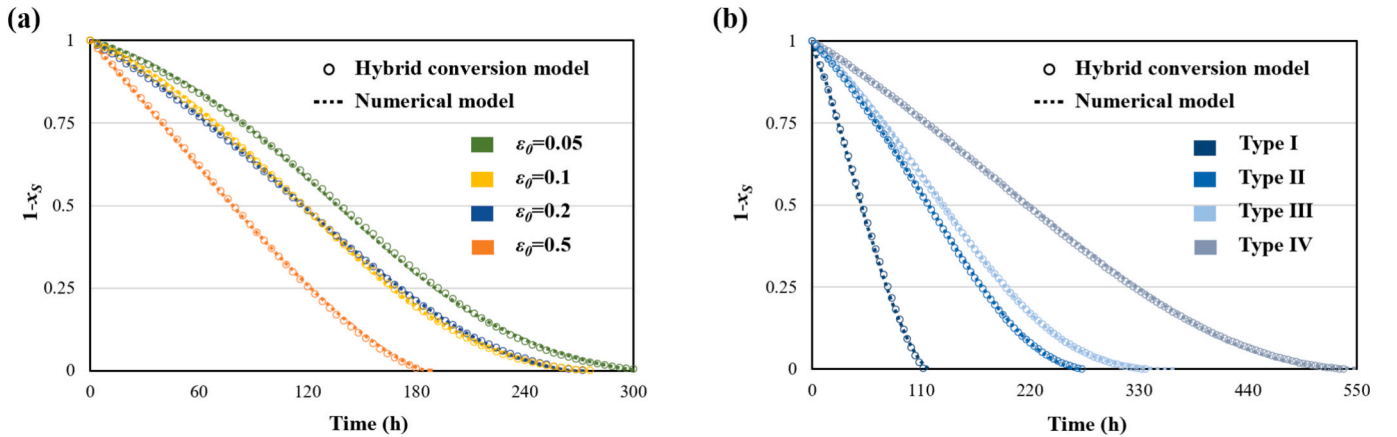
Fig. 8. Comparisons of remaining mass fraction curves from numerical model (micro-continuum approach) and hybrid conversion model across scenarios with varying (a) initial grain porosities and (b) reactive transport regimes.
