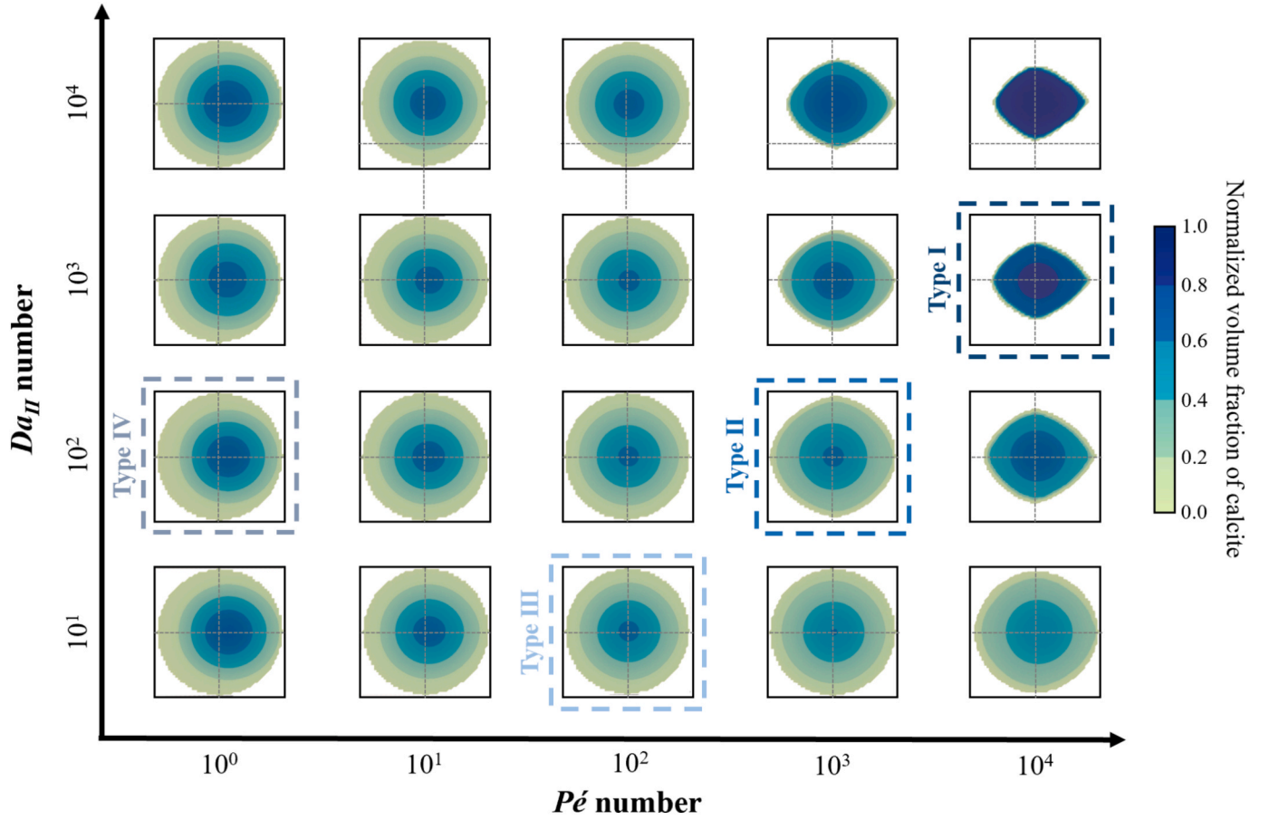
Fig. 4. Dissolution pattern diagram of porous grains ( \varepsilon_0 = 0.2 ) according to varying Pé and Da_{II} numbers. Time snapshots are selected for each scenario when the total volume fraction of calcite grains reaches 30 % with the flow from left to right. Regarding grain geometry and porosity distribution, four dissolution types are highlighted for further discussion.
