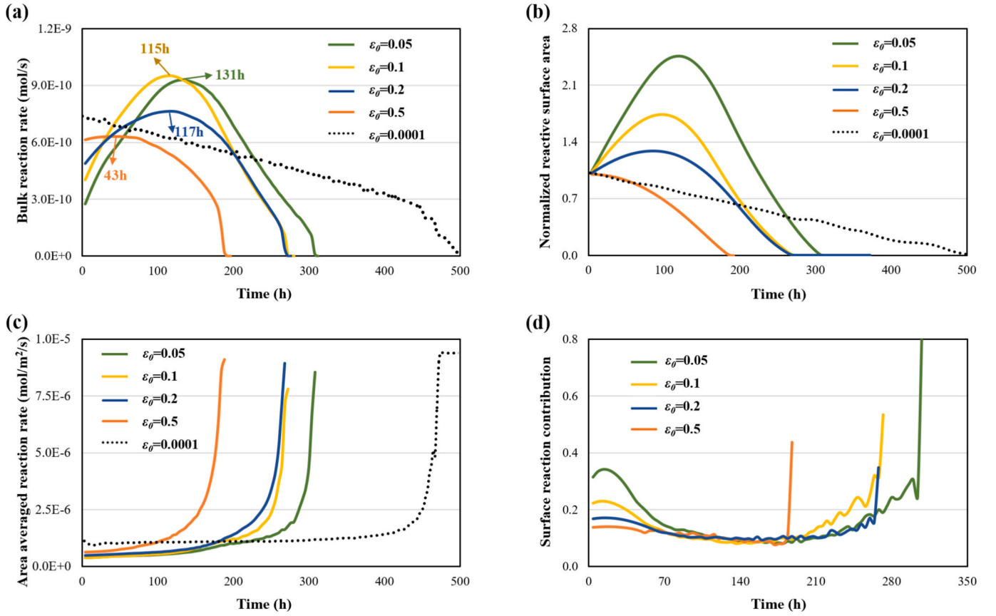
Fig. 3. Variations in (a) bulk reaction rate, (b) normalized reactive surface area (i.e., bulk surface area normalized against the initial value), (c) area-averaged reaction rate, and (d) relative contribution of surface reactions over time across simulation scenarios with different initial intragranular porosities. Colored arrows in Fig. 3a indicate the time points of maximum reaction rates. Surface reaction contribution is determined by the ratio of surface reaction rate (mol/s) to bulk reaction rate (mol/s). All simulation scenarios were conducted under the baseline reactive transport regime ( Pé \sim 10^3 , Da_{II} \sim 10^2 ), corresponding to the Type II regime described in the following discussion.
