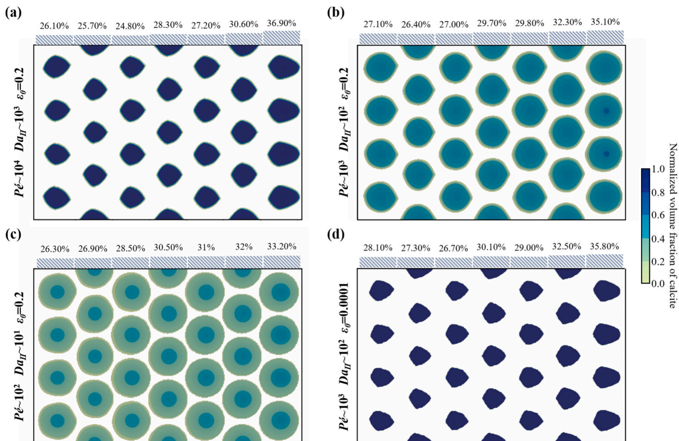
Fig. 10. Comparisons of spatial variations in calcite volume fraction across simulation scenarios with different reactive transport regimes and initial intragranular porosities. Fig. 10a–c illustrate porous grain-packing (each grain with a porosity of 0.2) dissolution under different reactive transport conditions, while Fig. 10d provides a comparison with the packing of impervious grains. Time snapshots are selected for each scenario when the overall volume fraction of calcite reaches 30%. The remaining volume fractions for each grain column are displayed at the top of subfigures.
