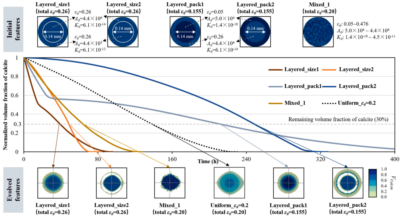
Fig. 9. Comparisons of calcite volume fraction evolution and spatial variations across simulation scenarios considering microcrystal-scale heterogeneities (Layered_size1/2: inner layer – fine/coarse microcrystal; Layered_pack1/2: inner layer – SCP/HCP). In these simulations, the flow velocity is 12 mm/s, the k_I is 0.89 mol/m 2 /s, and the Pé and Da_{II} are \sim 10^3 and \sim 10^3 , respectively. The surface area is calculated from A = \frac{6(1-\varepsilon)}{d} . The uniform case ( \varepsilon_0 = 0.2 ) serves as a reference under the same Pé and Da_{II} conditions. Time snapshots in the bottom panel are taken when the normalized calcite volume fraction reaches 30 % in each scenario.
