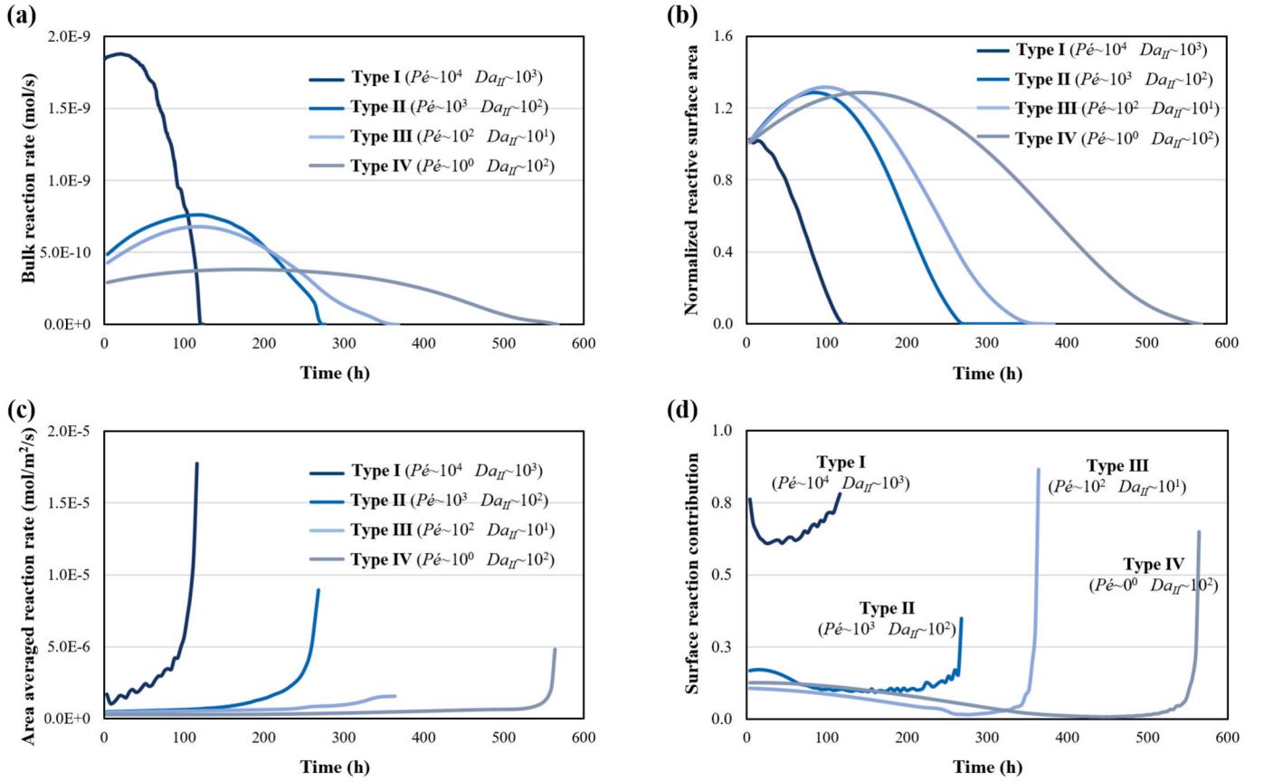
Fig. 5. Variations in (a) bulk reaction rate, (b) normalized reactive surface area, (c) surface area averaged reaction rate, and (d) relative contribution of surface reactions over time over time for different dissolution types selected based on Fig. 4.
