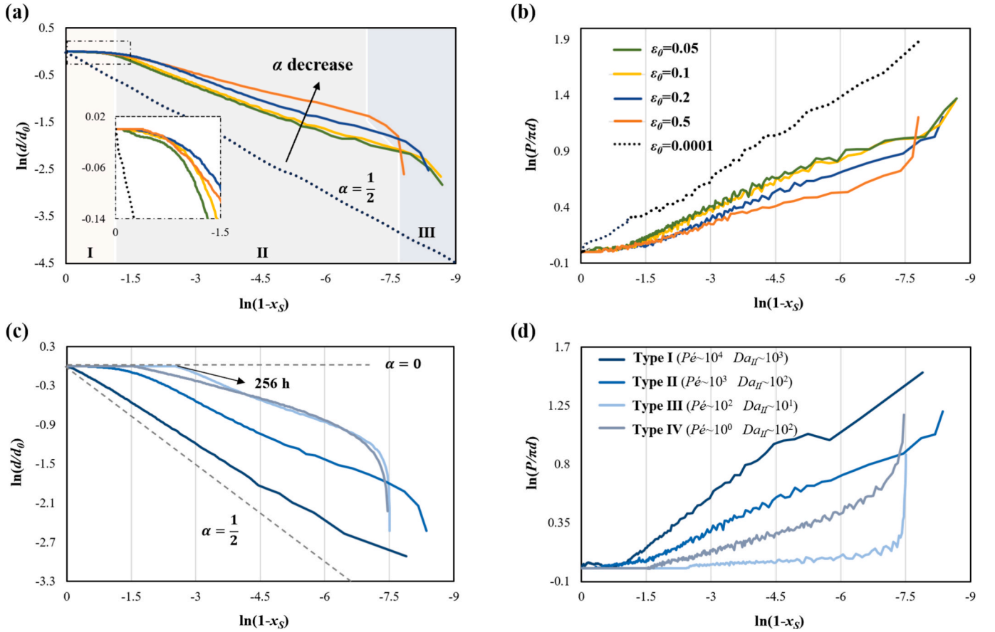
Fig. 7. Dependence of (a, c) grain equivalent diameter and (b, d) grain circularity on the reaction progression across simulation scenarios with different (a, b) initial porosities and (c, d) reactive transport regimes. In particular, the Type II transport regime was used for the simulations shown in Figs. 7a and 7b, and an initial porosity of \varepsilon_0 = 0.2 was set for the simulations in Figs. 7c and 7d. The exponents \alpha and \varphi correspond to the slopes of \ln - \ln plots shown in Figs. 7a and 7c, Figs. 7b and 7d, respectively. Three stages of reaction process highlighted in Fig. 7a, (i.e., I, II, and III) can be identified based to the dynamics of \alpha .
