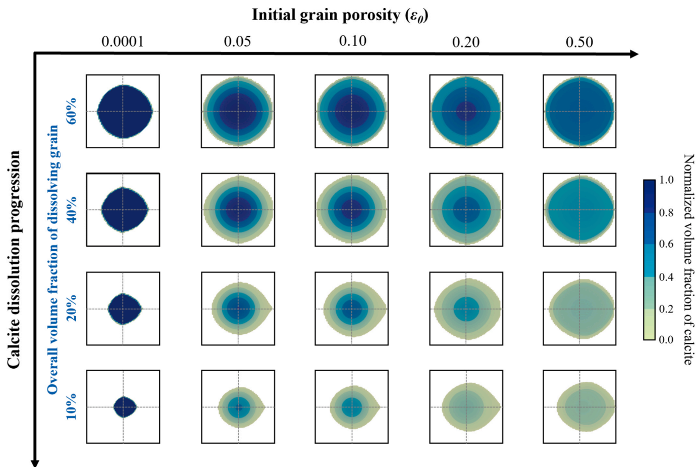
Fig. 2. Comparisons of spatial variations in calcite volume fraction across simulation scenarios with different initial intragranular porosities, ranging from impermeable ( \varepsilon_0 = 0.0001 ) to highly permeable (i.e., \varepsilon_0 = 0.05, 0.10, 0.20 , or 0.50 ) conditions. In these simulations, the flow proceeds from left to right at a velocity of 12 mm/s, with k_1 = 0.89 mol/m 2 /s. The corresponding Pé and Da_{II} numbers are \sim 10^3 and \sim 10^2 , respectively.
