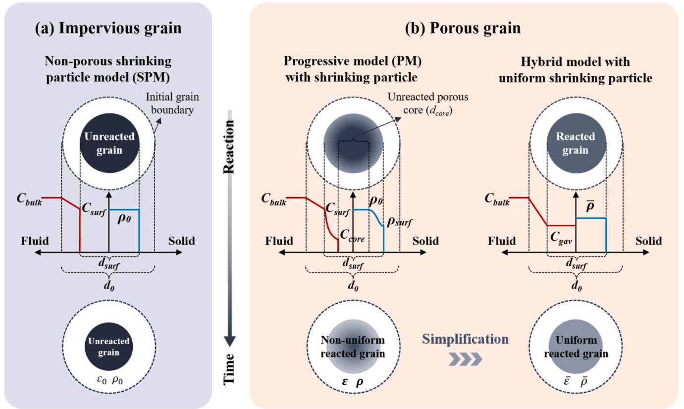
Fig. 6. Schematic illustration of altered grain structures according to different model assumptions for both (a) impervious and (b) porous cases. Herein, the subscripts bulk , surf , core , and gav denote bulk solution, grain surface, unreacted core surface and grain averaged value, respectively.
