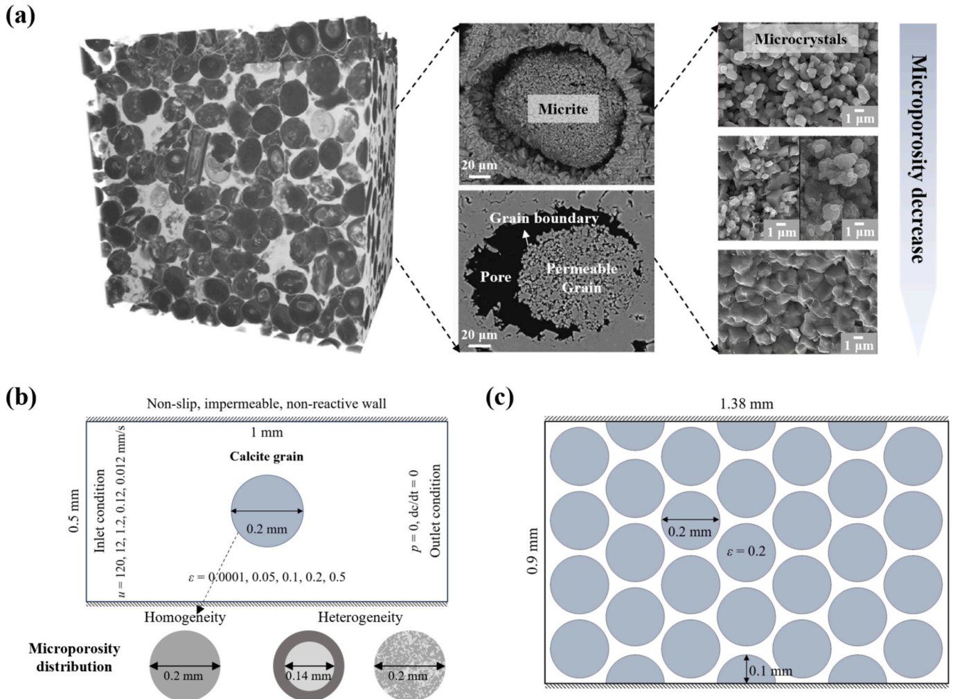
Fig. 1. Imaging of limestone pore structure and simulation setup. (a) Three-dimensional view of limestone modified after Mayo et al. (2015), with scanning electron microscopy images of micrite and microcrystals adapted from Noiriel et al. (2009) and Hashim & Kaczmarek (2019) (with permission from Elsevier). Computational domain—showing flow from left to right—along with the boundary and initial conditions for simulation scenarios, is illustrated for the (b) single-grain and (c) grain-packing sets. Spatial variations in microporosity, including both uniform and non-uniform distributions within a single grain, are illustrated in Fig. 1b. The greyscale represents various values of microporosity, and the model conceptualization is shown in Fig. S3.
