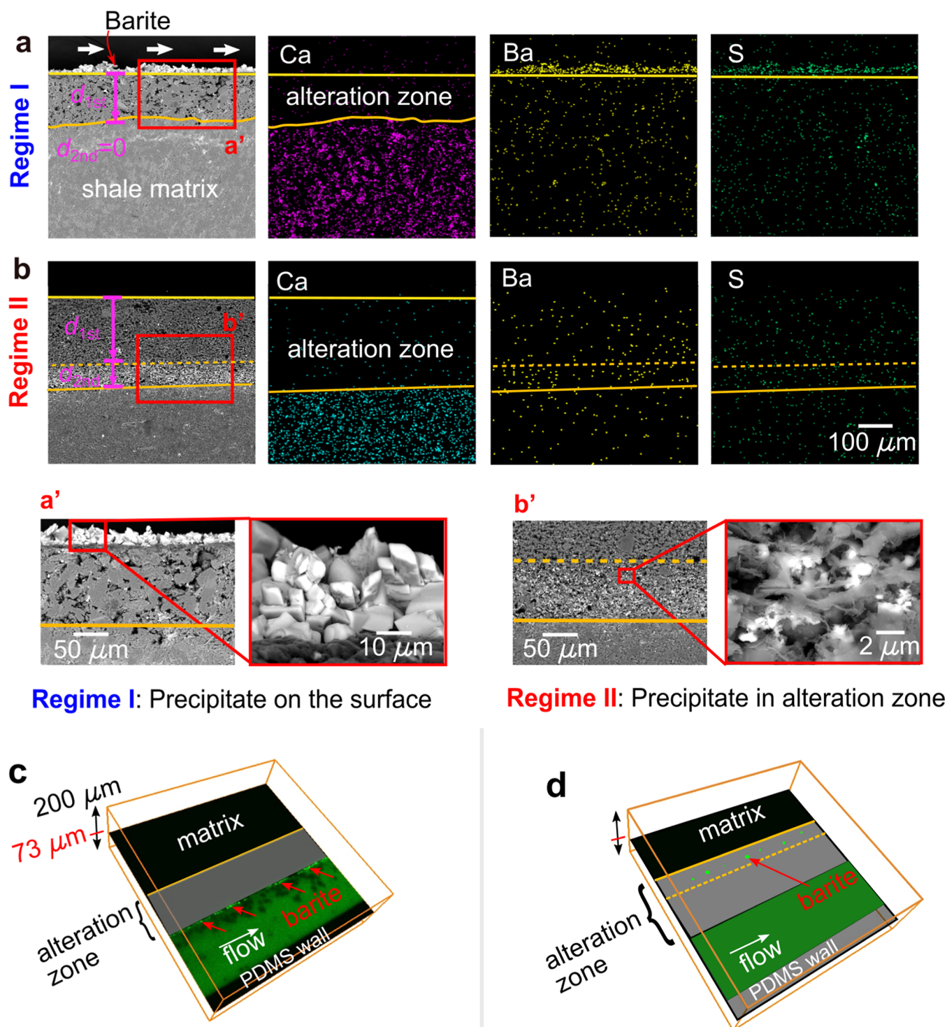
Figure 3. Observation of two precipitation regimes. (a) In regime I, a large amount of barite precipitation is observed with Pe = 107 and pH = 11 on shale surfaces by SEM-BSE images. These features of regime I is supported by the spatial distribution of elements (Ba, S) and the high-magnification SEM images (a'). According to the maps of various elements characterized by EDS, we can observe an obvious Ba element and S element gathered on the shale surface. Meanwhile, the extremely low content of Ca element confirms the alteration zone area. (b) In regime II, few barite precipitates are observed with Pe = 1067 and pH = 2 in the alteration zone formed during the second flooding. Ba element and S element are gathered but with the small amount in this secondary alteration zone. (c) Confocal microscopy images show significant precipitation-induced fluorescence accumulation on the shale wall (marked by red arrows) in the middle of the thickness direction ( 73 \mu\text{m} ). (d) Due to the opacity of the shale, the precipitation distribution of the precipitation regime II cannot be observed by confocal microscopy. A schematic diagram showing that the precipitation is mainly distributed in the secondary alteration zone. We verified the precipitation distribution of regime II by SEM-BSE characterization after grinding 30 \mu\text{m} surface of the shale piece down (Supporting Information Figure S9).
