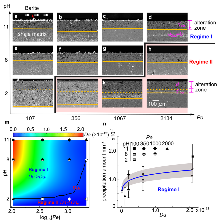
Figure 4. (a–l) Experimental phase diagram of precipitation regimes (I and II). The Pe number (or the flow rate v ) increases from the left to right. The pH increases from the bottom to the top. As the flow rate increases and pH decreases, the precipitation regime shifts from I [(a–g,i) precipitation on the shale surface] to II [(h,j–l) precipitation in the alteration zone]. (m) The transition of precipitation regimes is controlled by the dimensionless number Da . A threshold of Da can be obtained as Da_c \approx 1.05 \times 10^{-14} . For Da > Da_c , barite precipitates on the shale surface (regime I), while barite precipitation is observed in the alteration zone in the case of Da < Da_c . (n) In regime I, the amount of barite precipitation can be well corrected with Da using a power-law function a_{pre} = Da^{0.148 \pm 0.003} , indicating that increasing Da can promote the precipitation on the surface. The shadow denotes the 95% confidence interval.
