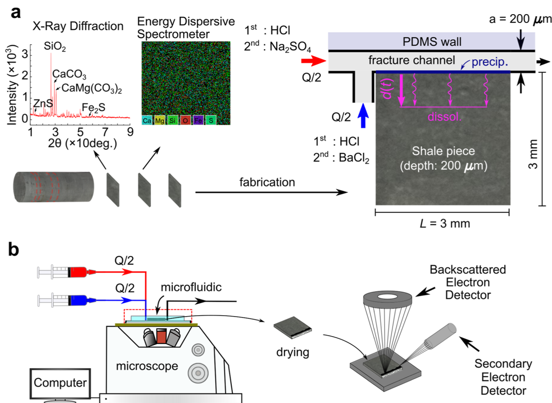
Figure 1. Shale microfluidic flow cell and experimental setup. (a) Mineral composition and sample preparation. The shale samples, characterized by X-ray diffraction (XRD) and scanning electron microscopy with energy-dispersive X-ray spectroscopy (SEM-EDS), mainly comprise quartz, dolomite, wurtzite, and calcite, with a minor amount of pyrite. Samples were cut from the same rock block into pieces with a size of 3 mm \times 3 mm and polished to a depth of 200 \mu\text{m} . In the PDMS flow cell, only one side (3 mm in length and 200 \mu\text{m} in depth) of the shale piece contacted the fluid. The fracture channel width b was approximately 200 \mu\text{m} . The detailed fabrication process of the microfluidic chip is shown in Supporting Information Figure S5. (b) Microfluidic-visualization system. The dissolution and precipitation processes were recorded using a fluorescence microscope. Postexperiment, shale samples were removed from the flow cells and examined in detail with scanning electron microscopy–backscattered electron detection (SEM-BSE).
