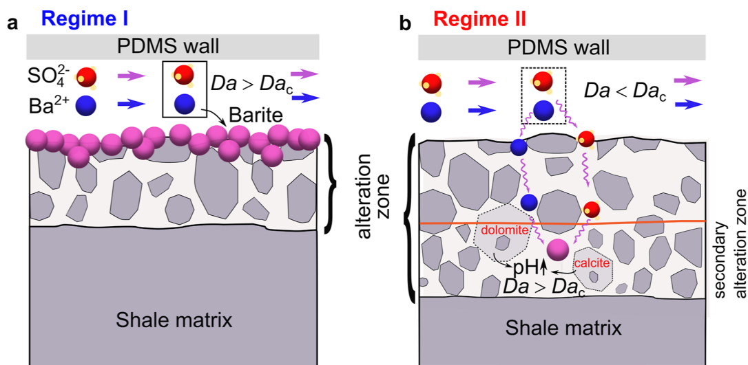
Figure 5. Mechanism of two precipitation regimes. (a) In regime I with a large Da number, which means faster precipitation rate, slower flow rate, and longer experimental time. Barite forms on the surface because it precipitates rapidly before diffusing inward, especially under conditions of high pH (where precipitation is much faster). In the experiment with pH = 2 and Pe = 107 , while the precipitation rate is relatively slower, barite precipitation on the fracture surface is observed because the long reaction time allowed a small amount of precipitation to accumulate on the surface. (b) In regime II with a low Da number, the precipitation rate is slower (at low pH) and the flow rate is faster and barite forms within the alteration zone. When the reactive fluid with Ba^{2+} and SO_4^{2-} at pH 2 diffuses to the calcite front, it reacts with carbonate minerals in the shale, increasing local pH and promoting barite precipitation in the alteration zone.
