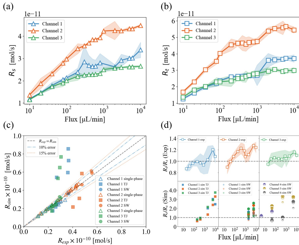
Figure 2. Experimental results of bulk reaction rate in (a) single-phase and (b) two-phase flow, (c) comparison of experimental and simulated bulk reaction rates, and (d) ratio of bulk reaction rates between two-phase and single-phase flow at the same total flow rate. Markers with reduced size and color saturation in (d) denote simulations with smaller slug length (see Table S2 in Supporting Information S1). The shaded areas in (a) and (b) show one standard deviation ( \sigma_{R_t} and \sigma_{R_s} ) of the effluent measurements, and in (d) it shows the standard deviation of R_t/R_s defined as \sigma_{ratio} = \frac{R_t}{R_s} \times \sqrt{\left(\frac{\sigma_{R_t}}{R_t}\right)^2 + \left(\frac{\sigma_{R_s}}{R_s}\right)^2} .
