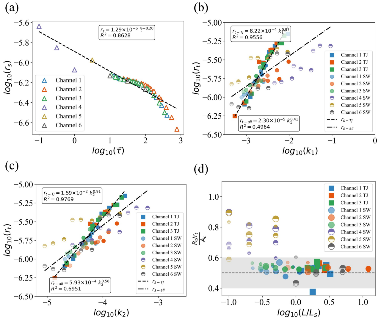
Figure 4. (a) Surface area averaged reaction rate in single-phase flow in relation to \bar{\tau} , surface area averaged reaction rate in two-phase flow in relation to (b) k_1 and (c) k_2 , and (d) effective surface area over geometric surface area in relation to L/L_s . Larger markers in (d) represent higher flow rates, and lower color saturation represent smaller slug size.
