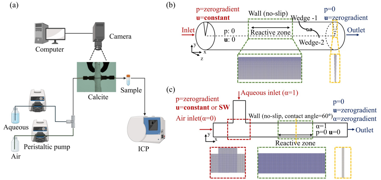
Figure 1. (a) Schematic of the experimental setup, and illustration of the geometry and meshing used in the (b) single-phase and (c) two-phase flow reactive transport simulations.
