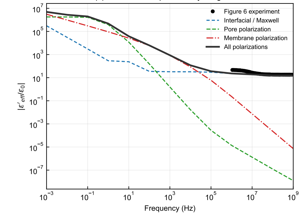
(c) Real relative permittivity magnitude
