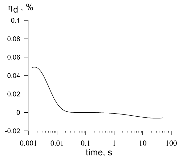
Fig. 5. Apparent differential polarizability obtained on the water. Note that when t > 0.02 s, the apparent differential polarizability becomes lower than 0.01%. Low values stipulated by the electrode polarization confirm accuracy of the measurement setup.
