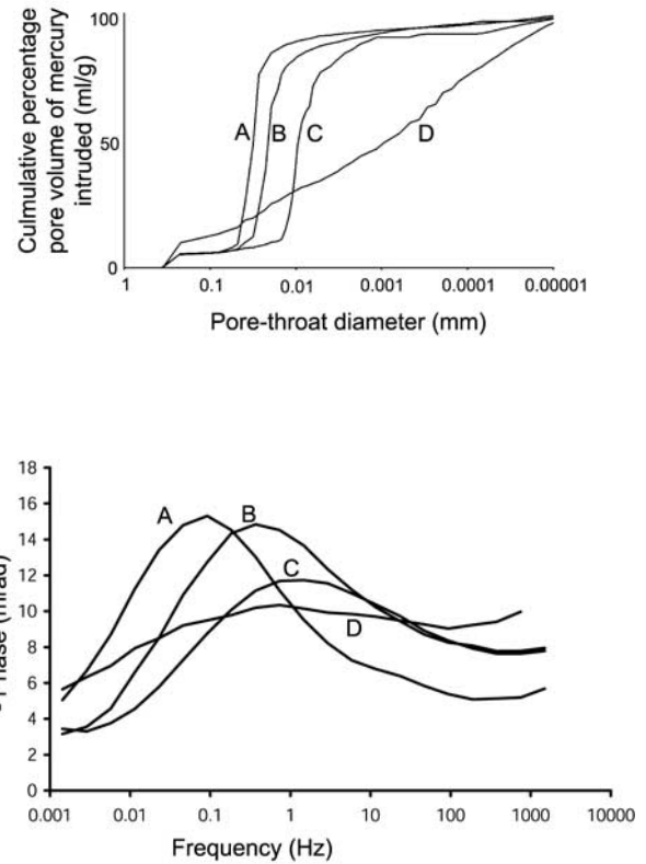
Figure 3. A comparison of pore-throat size with phase spectra of four Triassic sandstone samples A, B, C and D, taken from a 50 m borehole at the University of Birmingham, central England. (a) MICP cumulative pore-throat size distribution. (b) Low-frequency phase spectra from electrical measurements.
