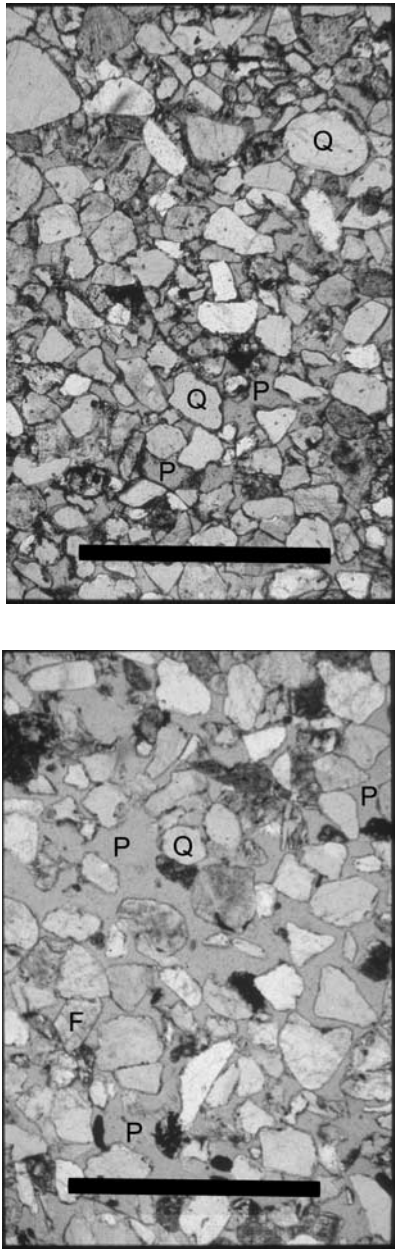
Figure 2. Thin sections of Triassic sandstone samples with 1 mm black scale bar. (a) Sample from Kirkham, Northwest England. An aquifer rock associated with the East Irish Sea basin. (b) Sample from Selby, Northeast England. An aquifer rock associated with the North Sea Basin. Pore space (P), Quartz grain (Q), Feldspar (F).
