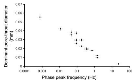
Figure 4. Dominant pore-throat diameter from MICP against the frequency value of the phase peak from electrical measurements. The results of all sandstones measured that had a dominant pore-throat size and a well-defined phase peak.
