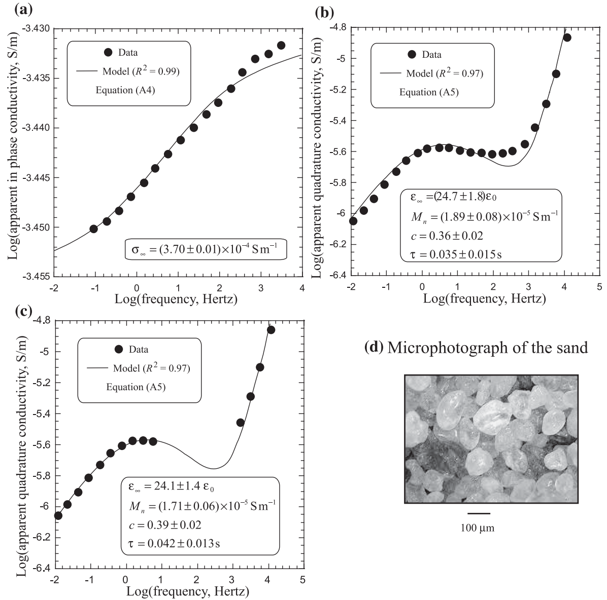
Figure 3. In-phase and quadrature conductivities of a clean sand with a very narrow grain size distribution with a mean diameter of 100 \mu\text{m} (data from Vaudelet et al. 2011a). (a), (b) For the quadrature conductivity, the data comprised between the low-frequency peak of the spectrum and the high-frequency dielectric effect is not fitted because of the potential effect of the roughness of the grain-pore water interface in this domain as shown in Fig. 2. \epsilon_0 denotes the dielectric constant of vacuum. (c) Fit of the quadrature conductivities data from Vaudelet et al. (2011a) not taking into account the data potentially influenced by the roughness of the grains. Grain diameter 100 \mu\text{m} , formation factor 3.1 and permeability 2.85 \times 10^{-12} \text{ m}^2 . The pore size of the sand is roughly 8.4 \mu\text{m} . (d) Microphotograph of the sand.
