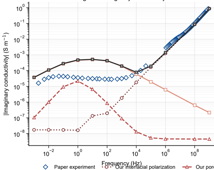
Figure 8: imaginary conductivity
