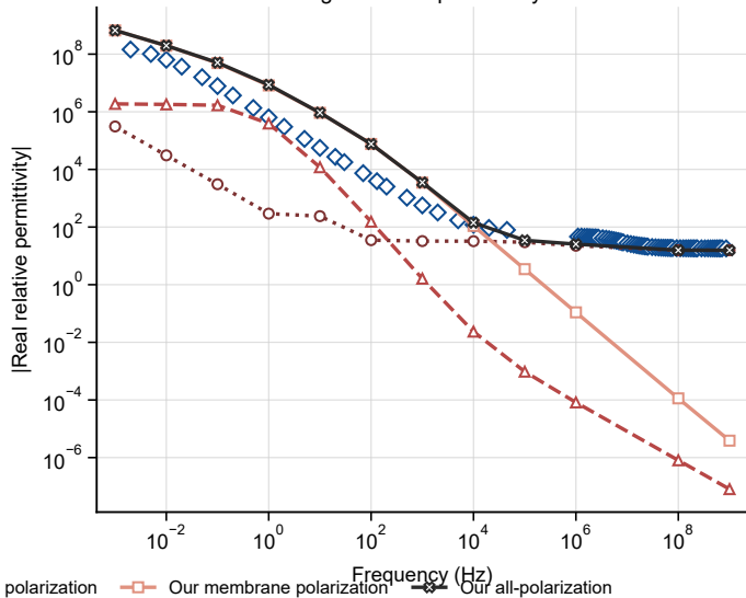
Figure 8: real permittivity
