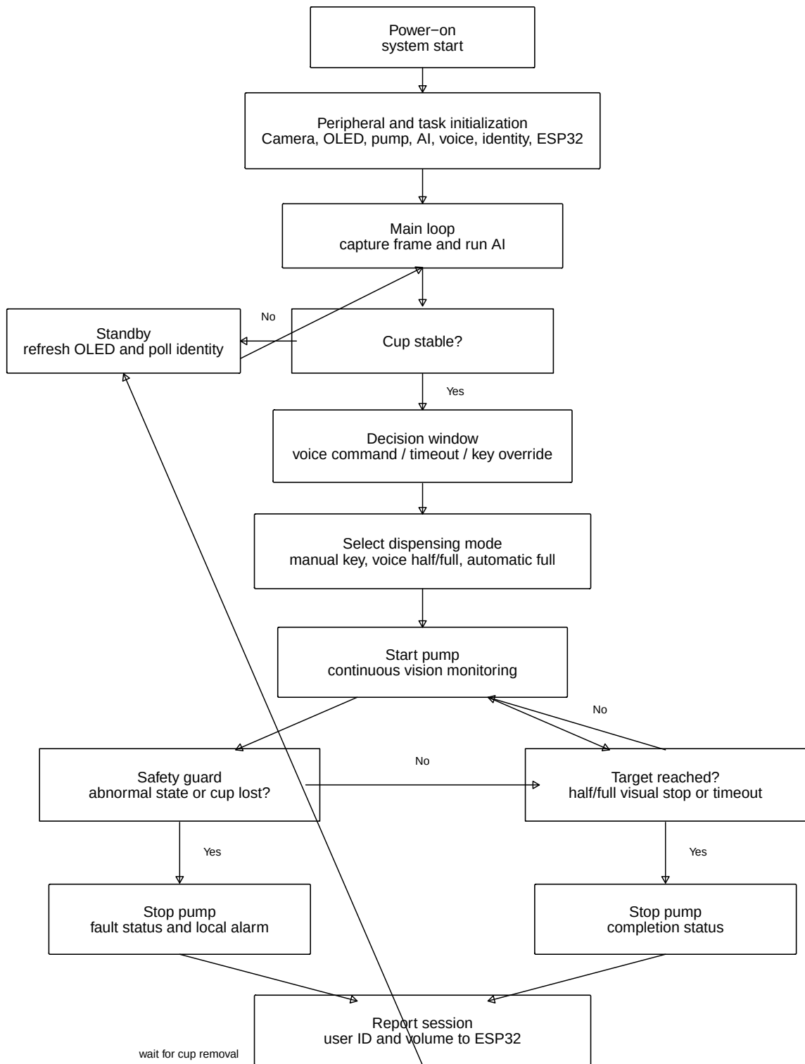
Fig. X. Main software workflow. The identity result is supplementary and does not block dispensing.
