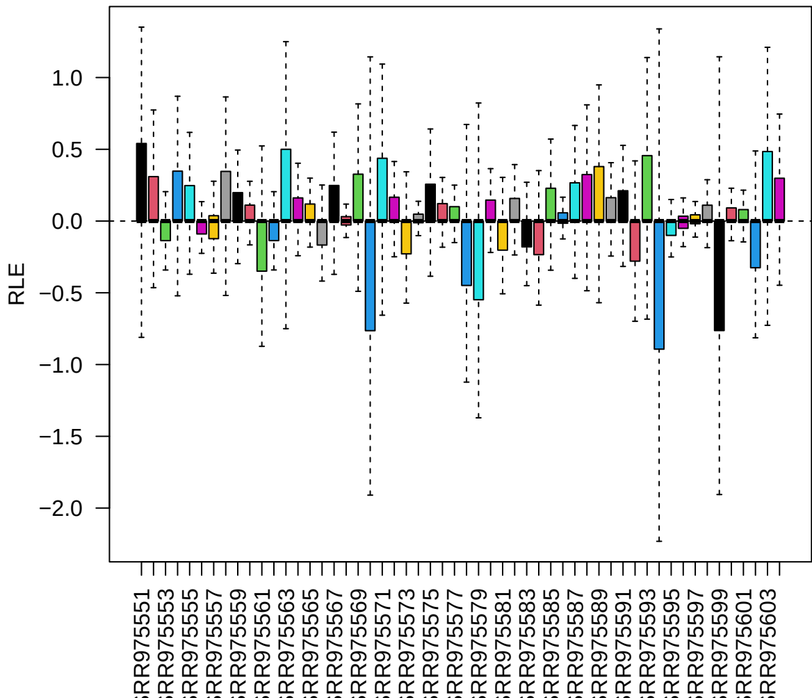
RLE of raw counts
