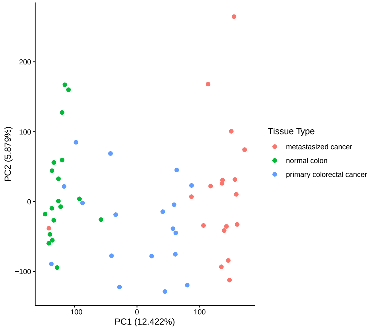
PCA of raw counts (log1p)
