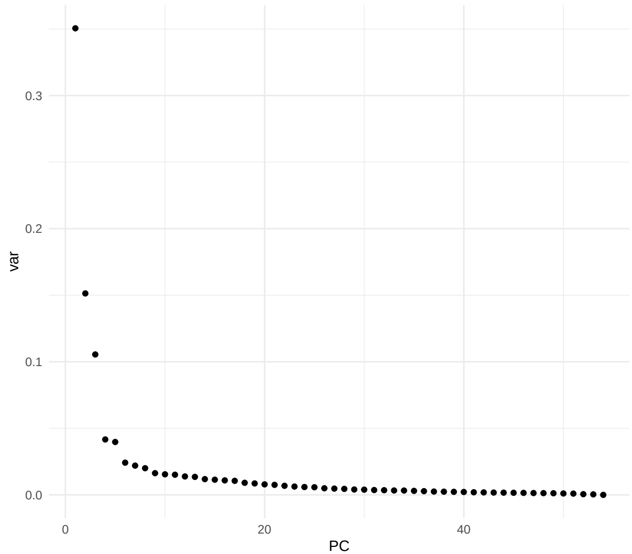
PCA Scree Plot – TMM Normalized
